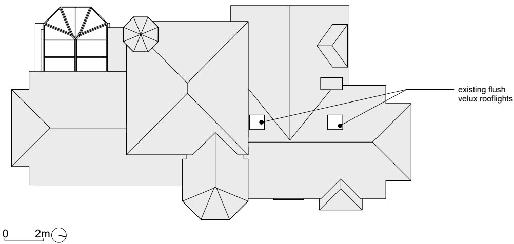
1 Roofplan Existing 1 : 200
