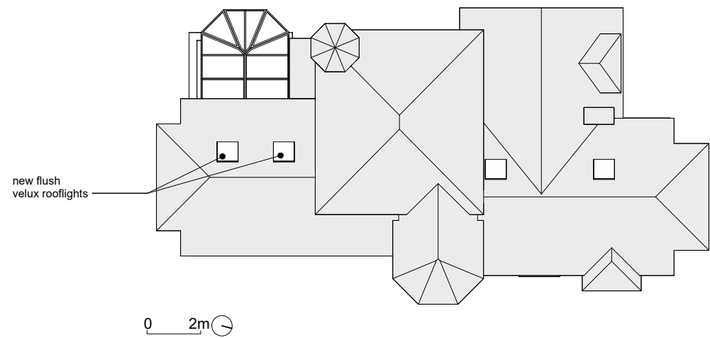
2 Roofplan Proposed 1 : 200
