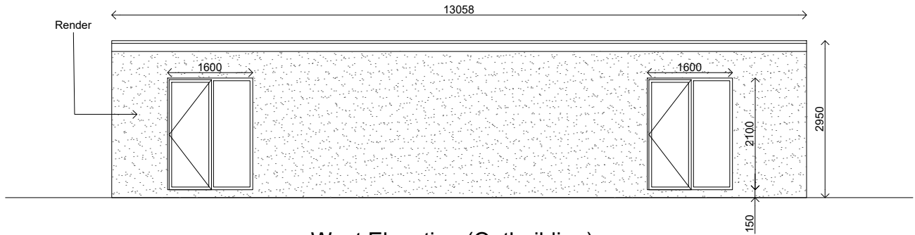
West Elevation (Outbuilding)
