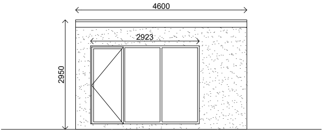
South Elevation (Outbuilding)
