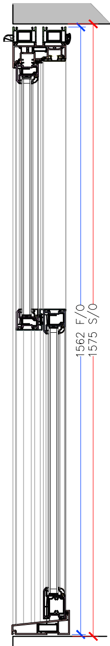
SECTION AA SCALE 1:10
