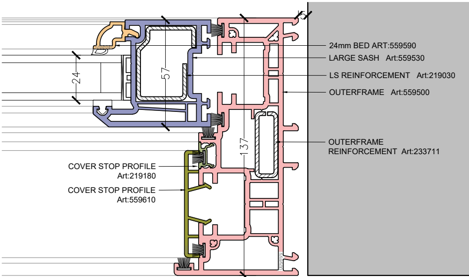
SECTION B SCALE 1:2
