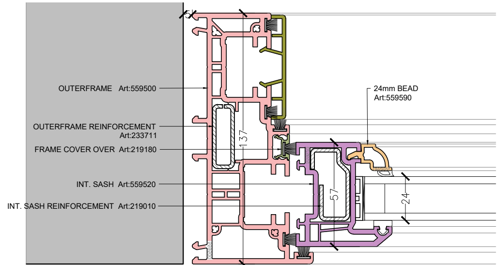
SECTION C SCALE 1:2
