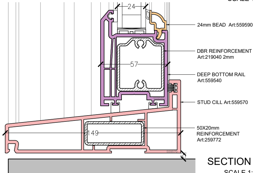
SECTION F SCALE 1:10
