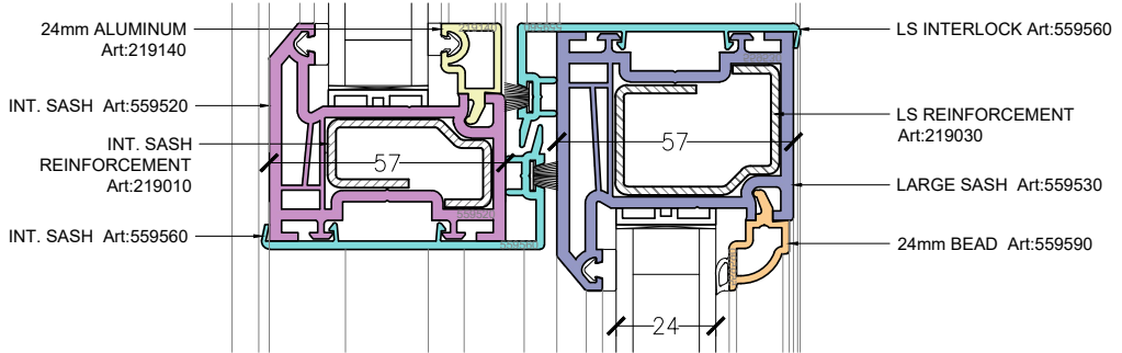
SECTION F SCALE 1:10
