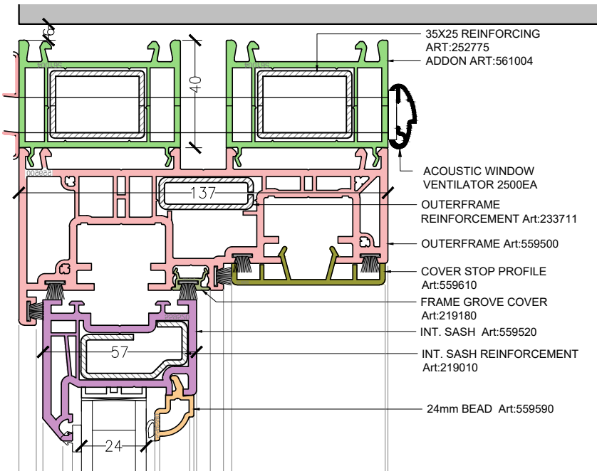
SECTION G SCALE 1:10
