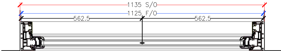
SECTION BB SCALE 1:10
