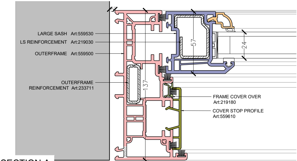
SECTION A SCALE 1:2
