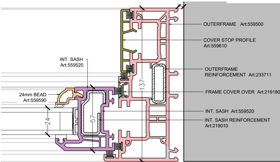
SECTION D SCALE 1:2
