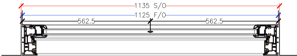
SECTION CC SCALE 1:10
