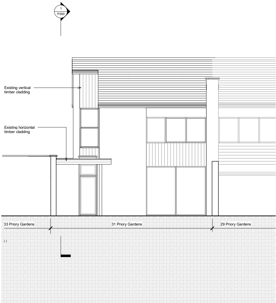
1 Existing South Elevation 1 : 50
