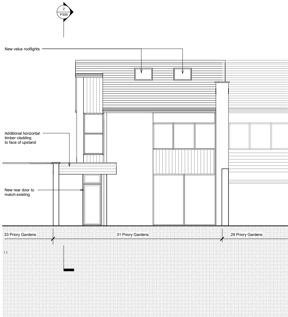
2 Proposed South Elevation 1 : 50
