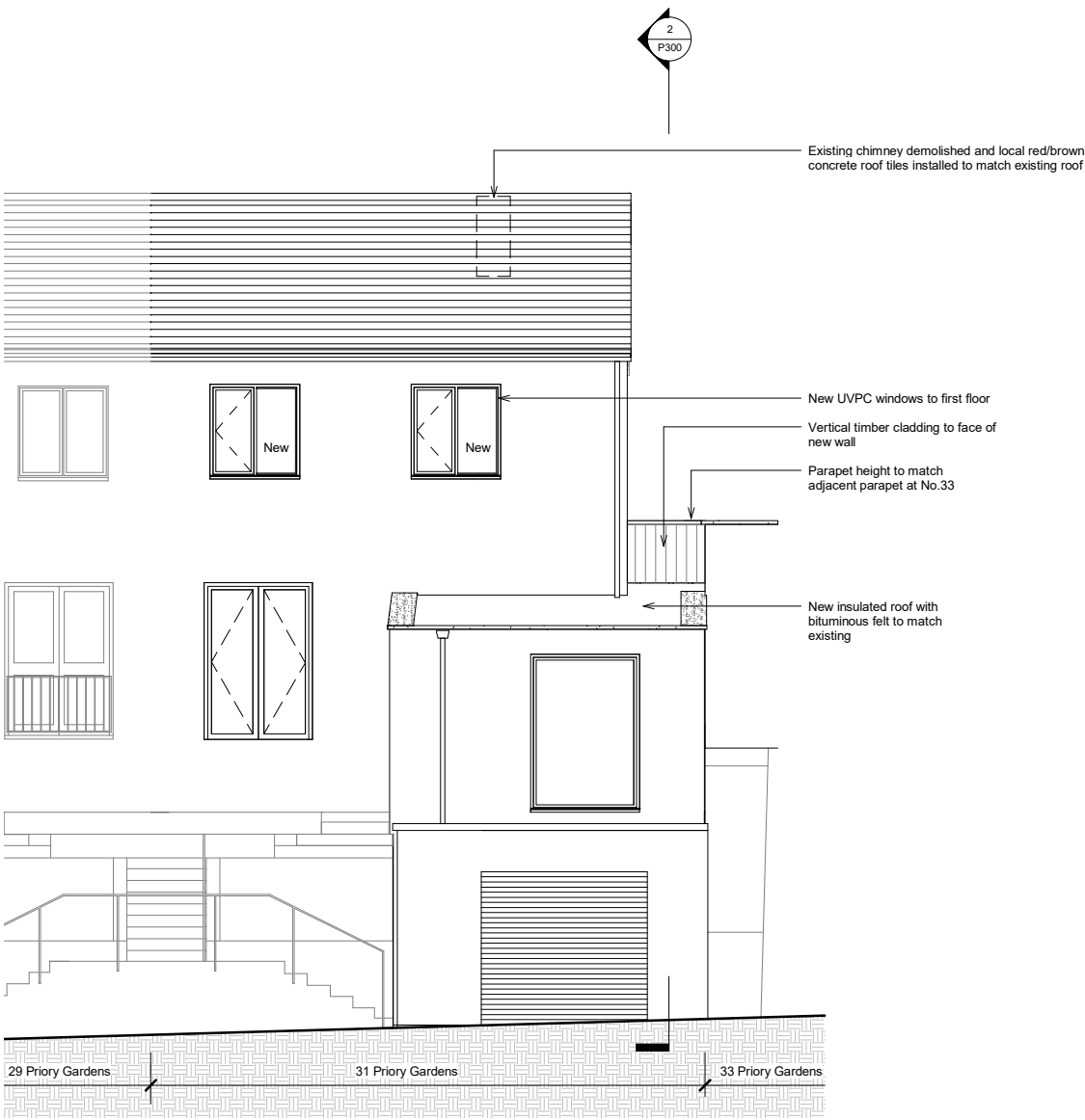
2 Proposed North Elevation 1 : 50
