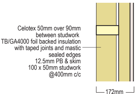
Drop Wall Detail 1
