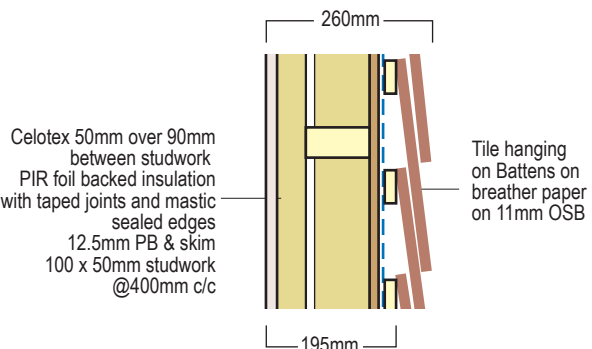
Dormer Wall Detail 4 U=0.18
