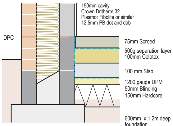
Ground Floor Slab U=0.18 Wall U=0.18
