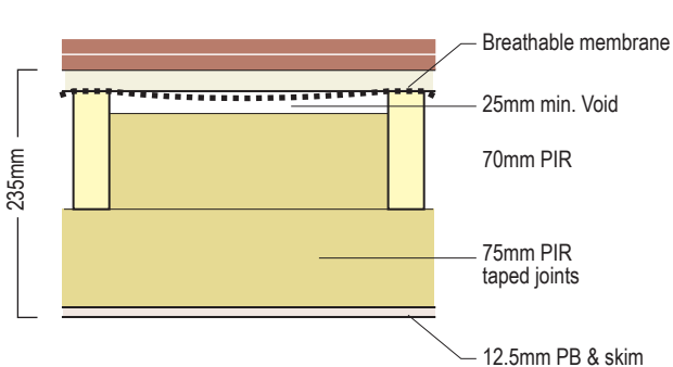
Sloping Ceiling Detail 2
