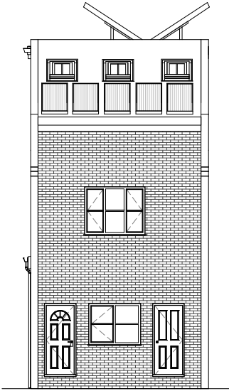
FRONT ELEVATION SOUTH
