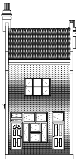
SOUTH ELEVATION
