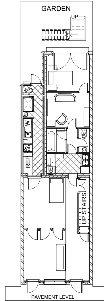
PAVEMENT LEVEL GROUND FLOOR PLAN
