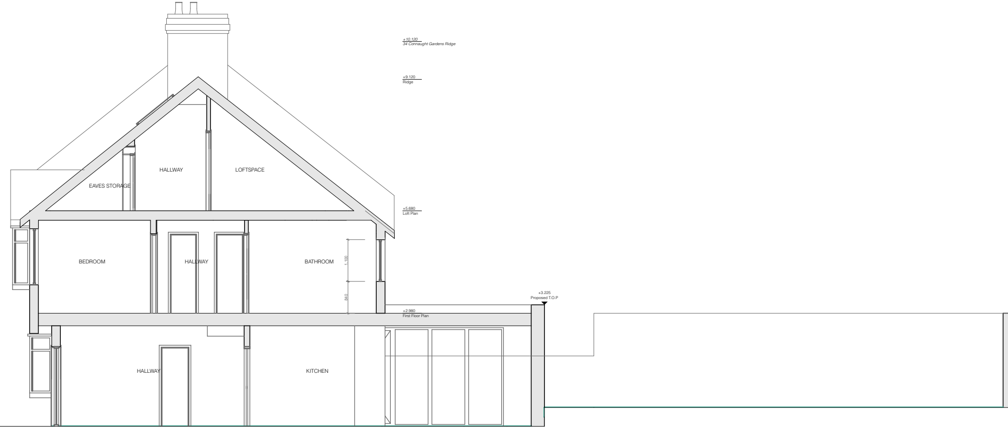
Section AA 1:100
