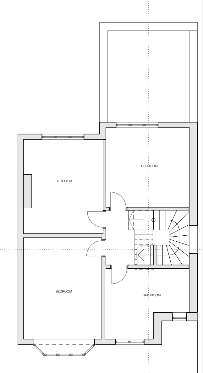
First Floor 1:100
