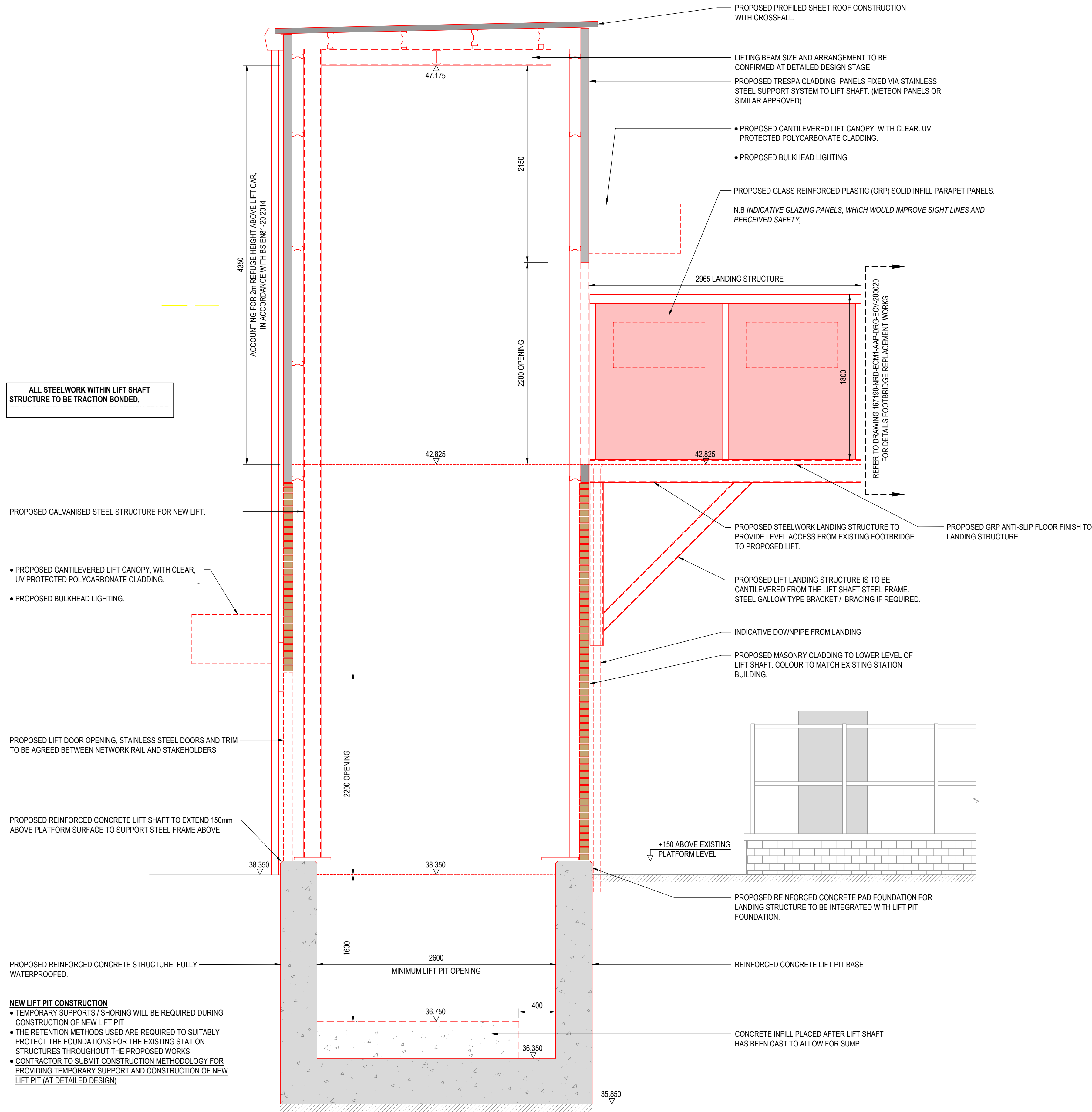
SECTIONAL ELEVATION THROUGH PROPOSED LIFT AND LANDING (PLATFORM 2) SCALE 1:25
