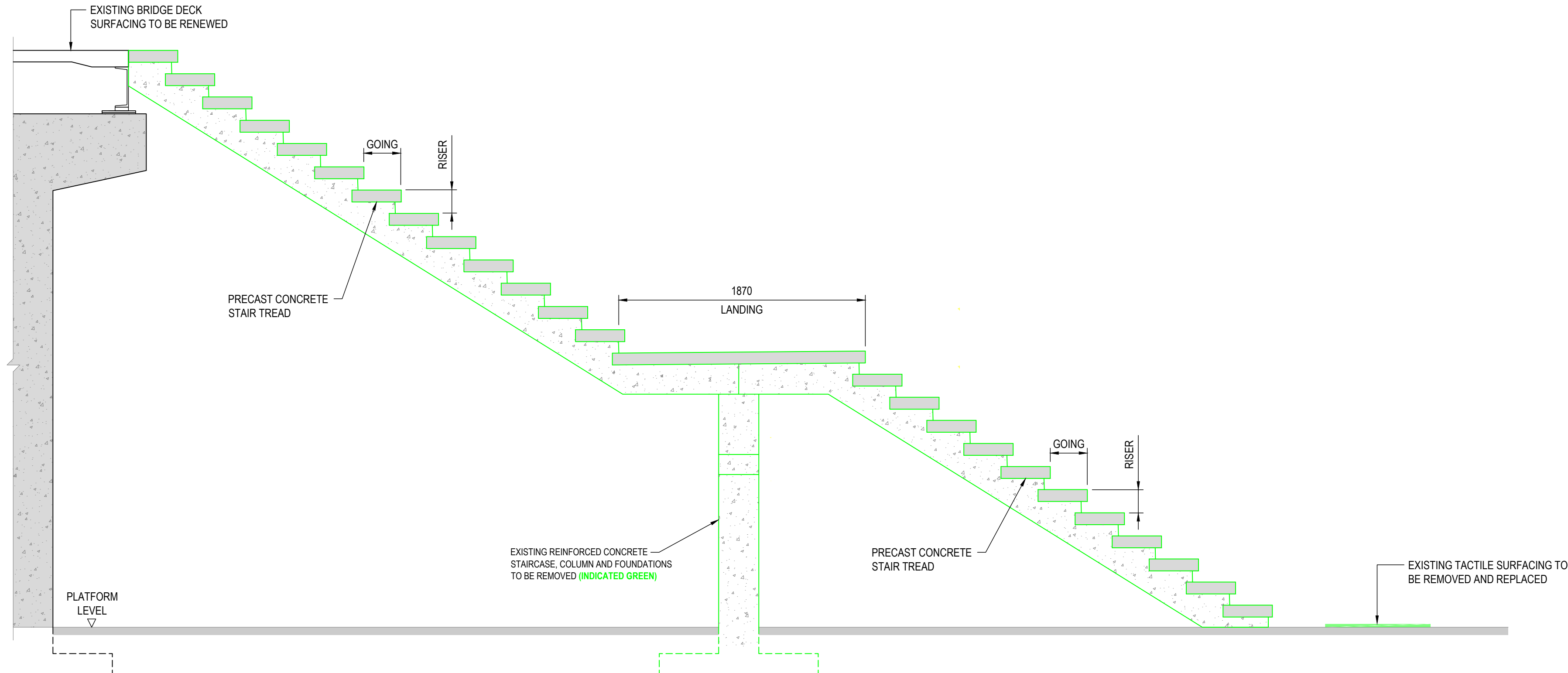
SECTION THROUGH EXISTING STAIRCASE (PLATFORM 3 & 4) SCALE 1:25
