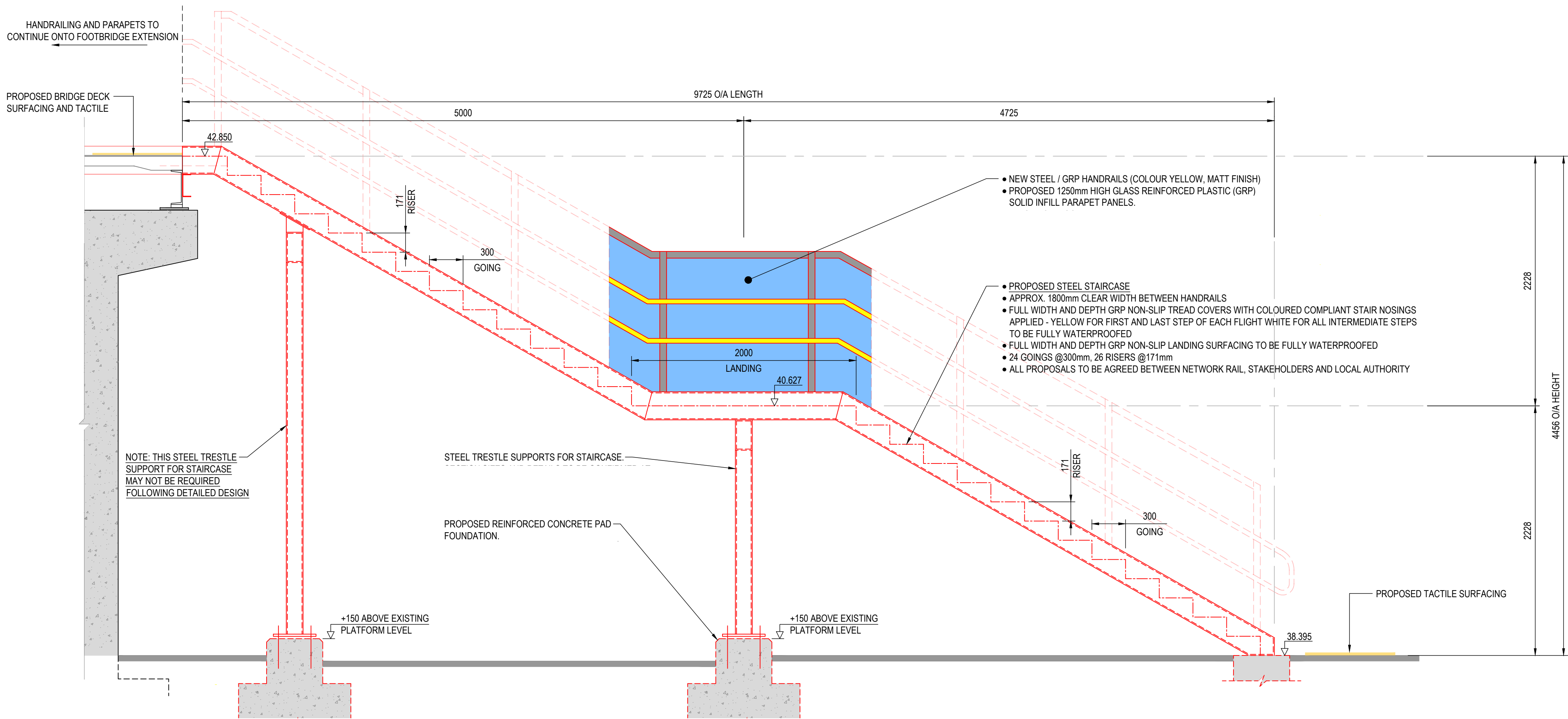
SECTION THROUGH PROPOSED STAIRCASE (PLATFORM 3 & 4) SCALE 1:25
