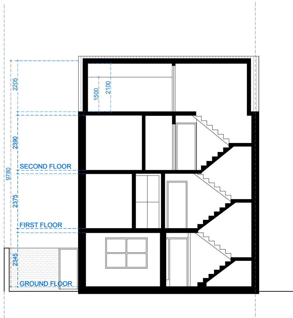
SECTION AA
