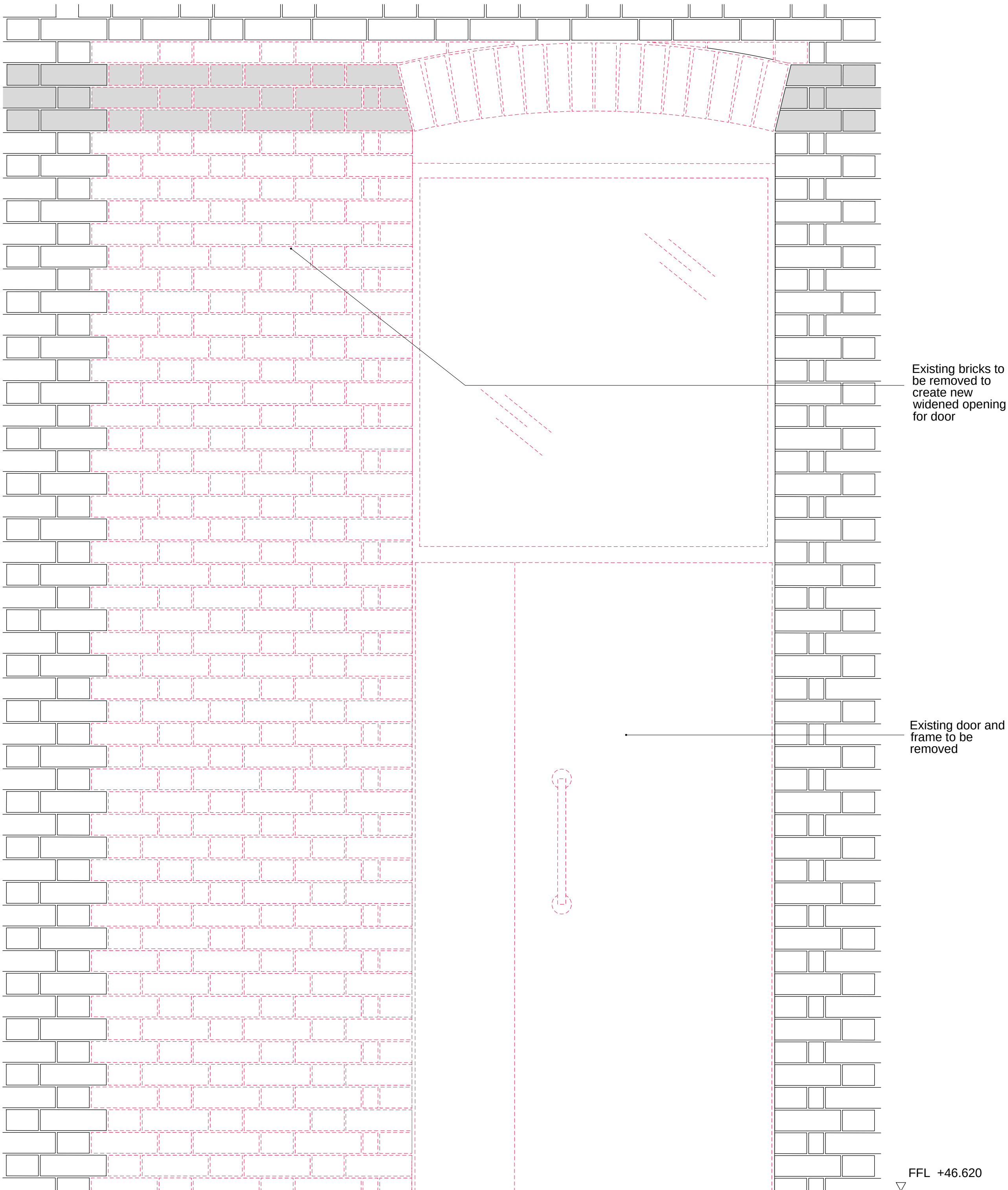
01 D-G-09 - Existing elevation with alterations 1:10
