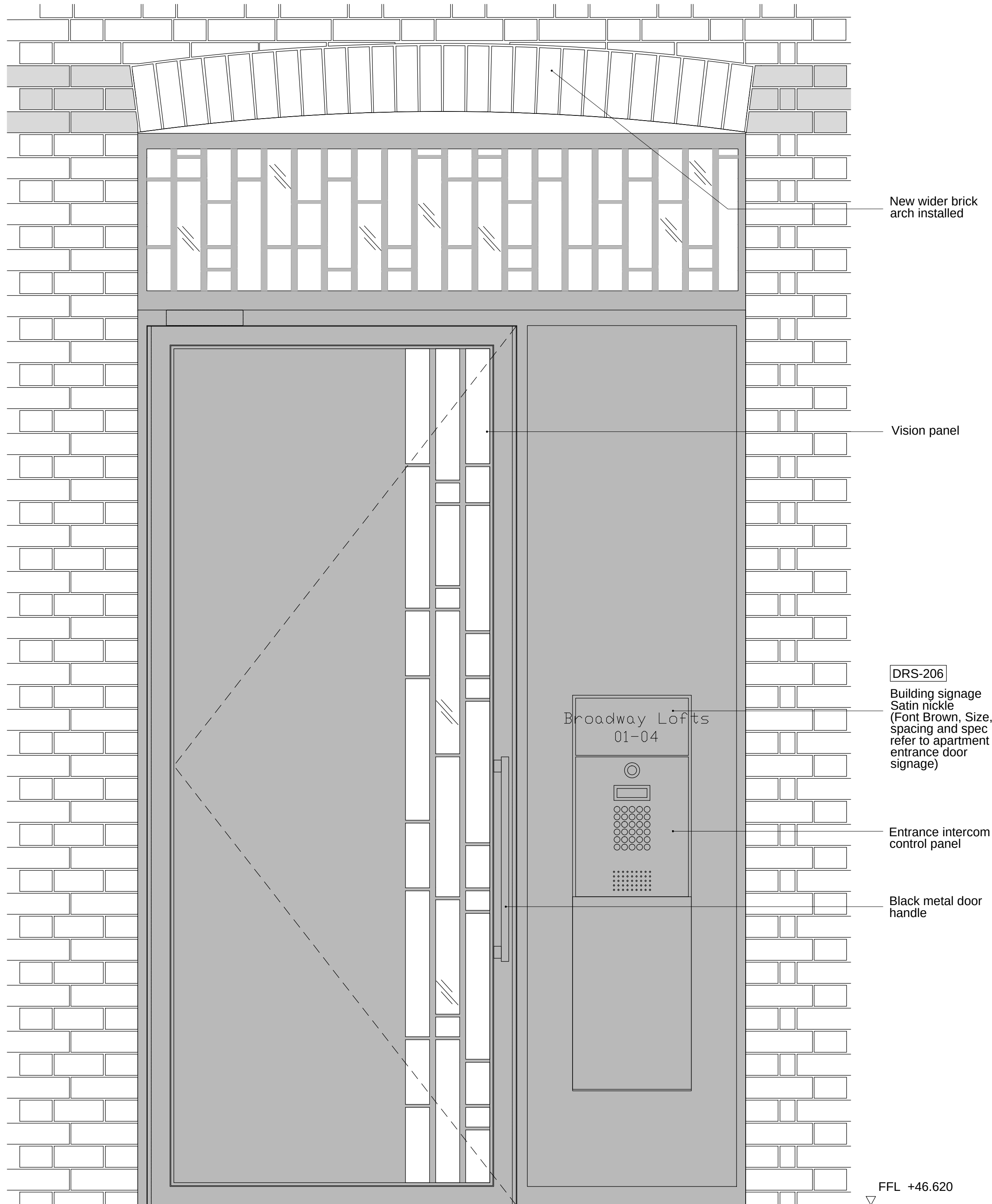
02 D-G-09 - Proposed elevation 1:10
