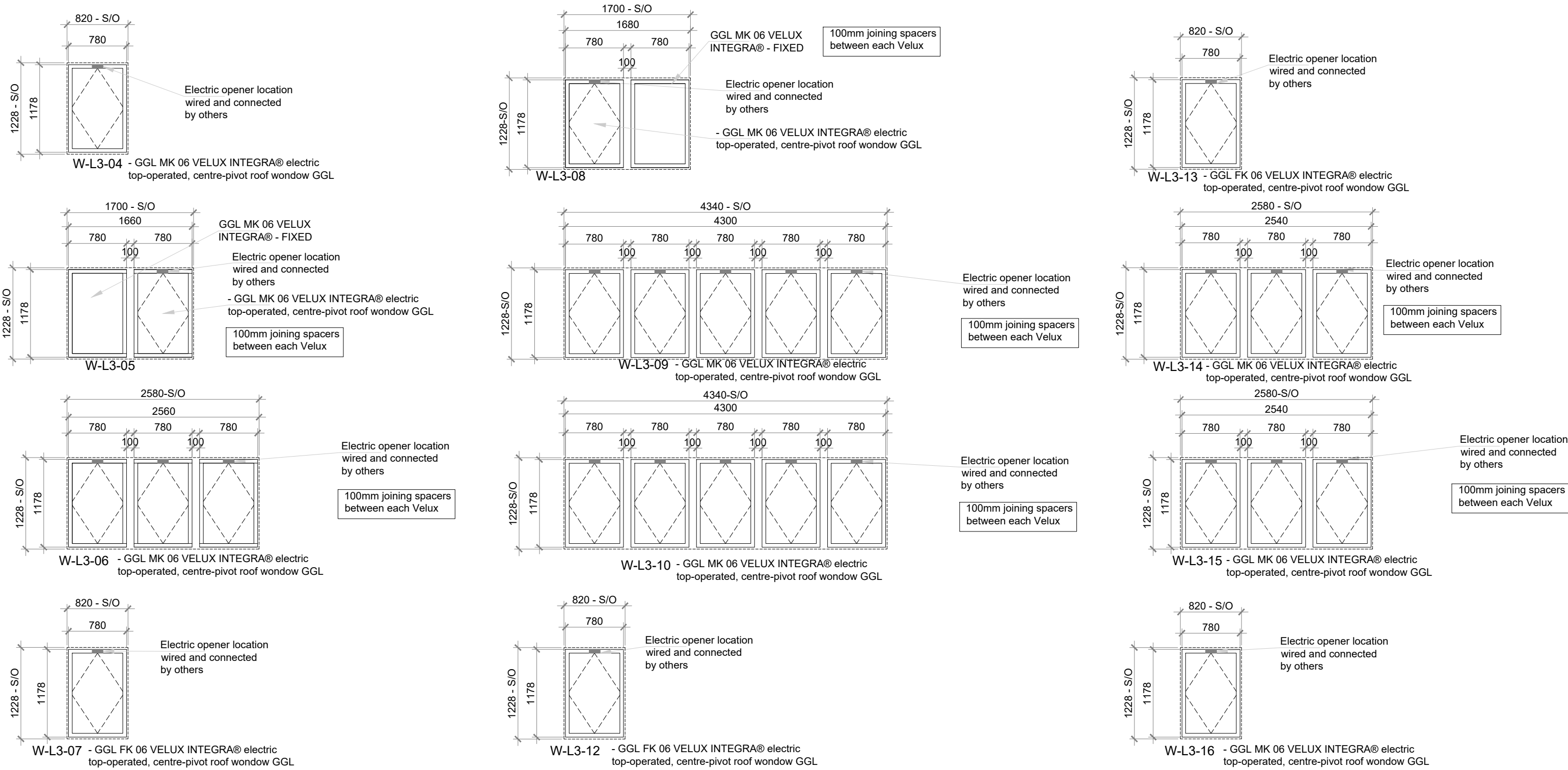
HORNSEY TOWN HALL - ROOF LIGHT SCHEDULE
