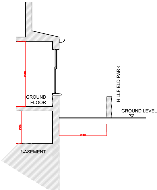
EXISTING SECTION
