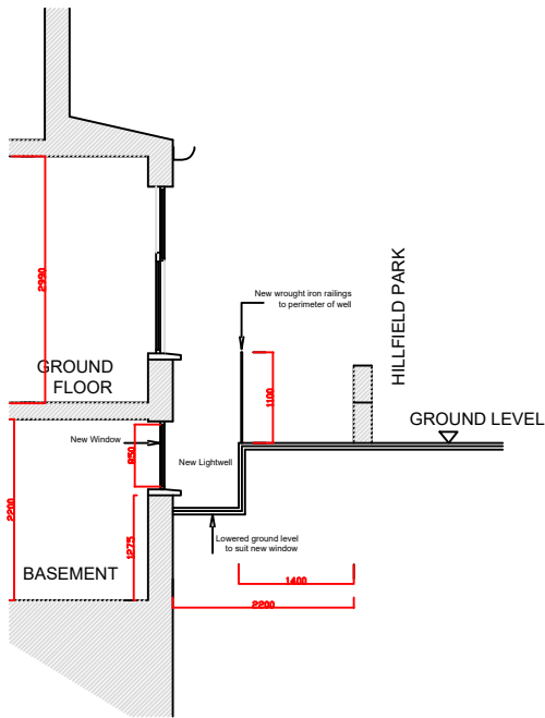
PROPOSED SECTION
