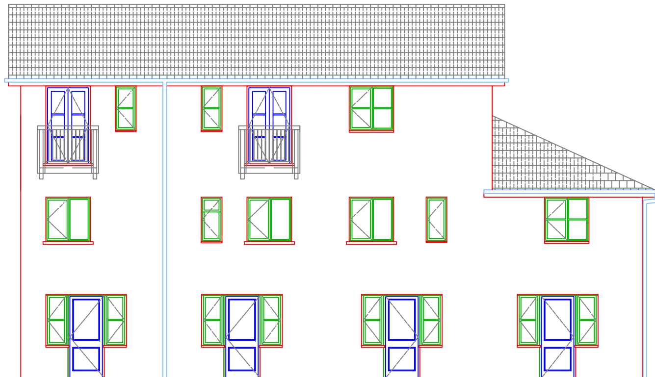
REAR ELEVATION
