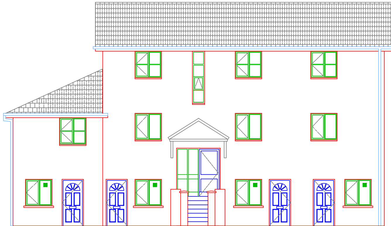
FRONT ELEVATION
