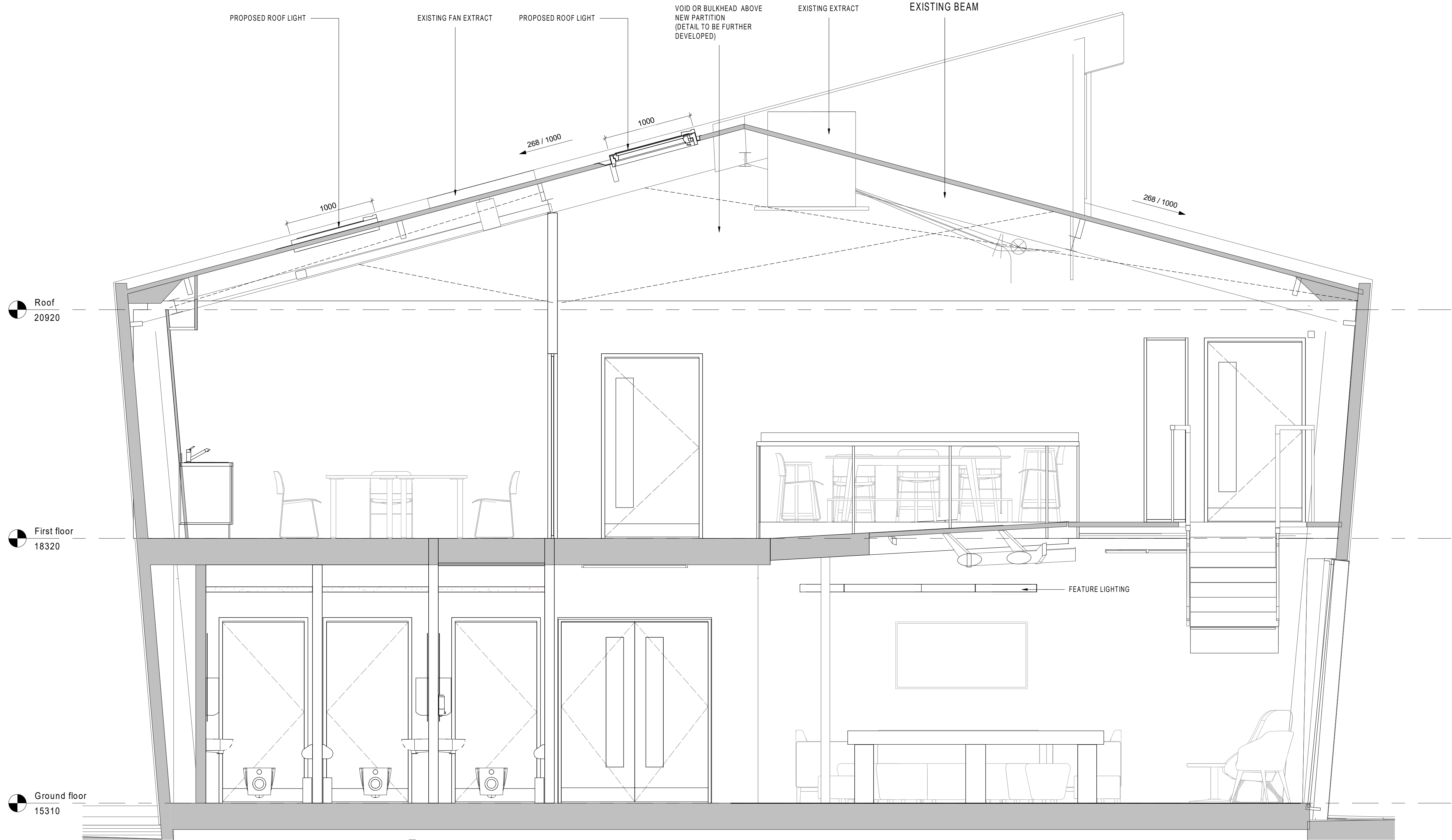
1 PROPOSED SHORT SECTION AA 1 : 25
