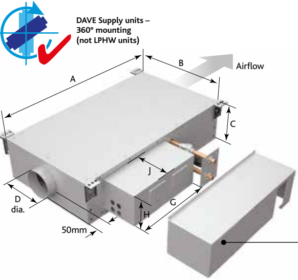
SUPPLY FAN SIZE DS6 - DATA LPHW 82/71 (Deg C)
