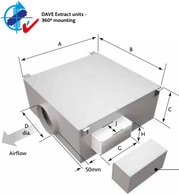
EXTRACT FAN SIZE DE4 - DIMENSIONS (mm)
