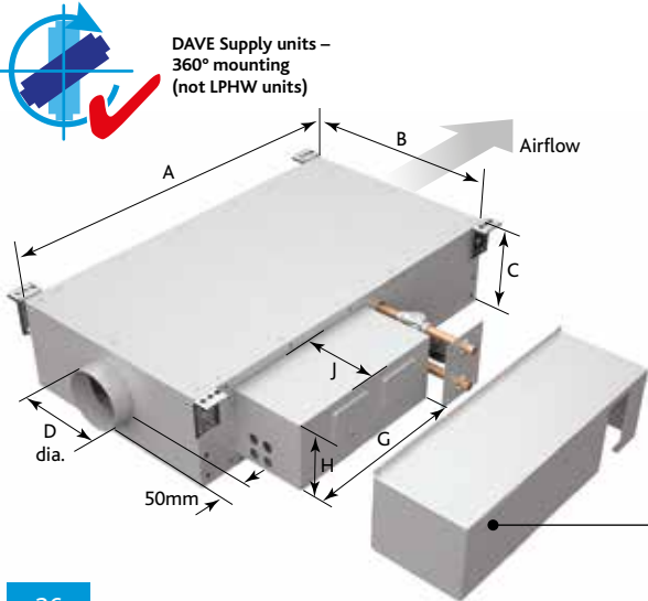
SUPPLY FAN SIZE DS4 - DATA LPHW 82/71 (Deg C)
