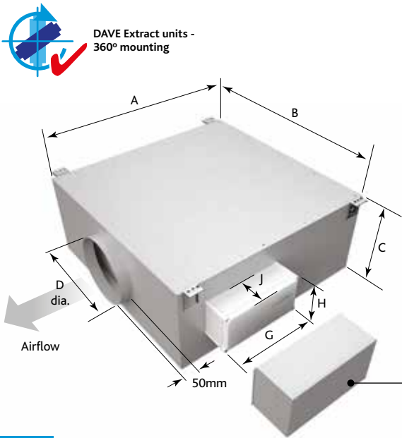
EXTRACT FAN SIZE DE2 - DIMENSIONS (mm)
