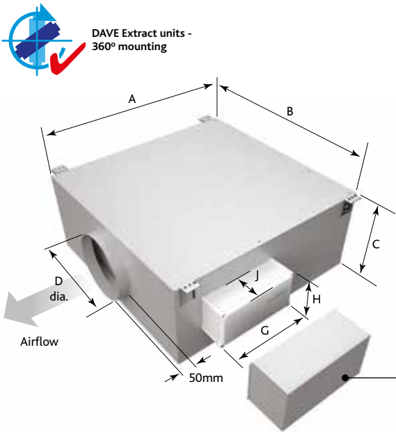
EXTRACT FAN SIZE DE5 - DIMENSIONS (mm)
