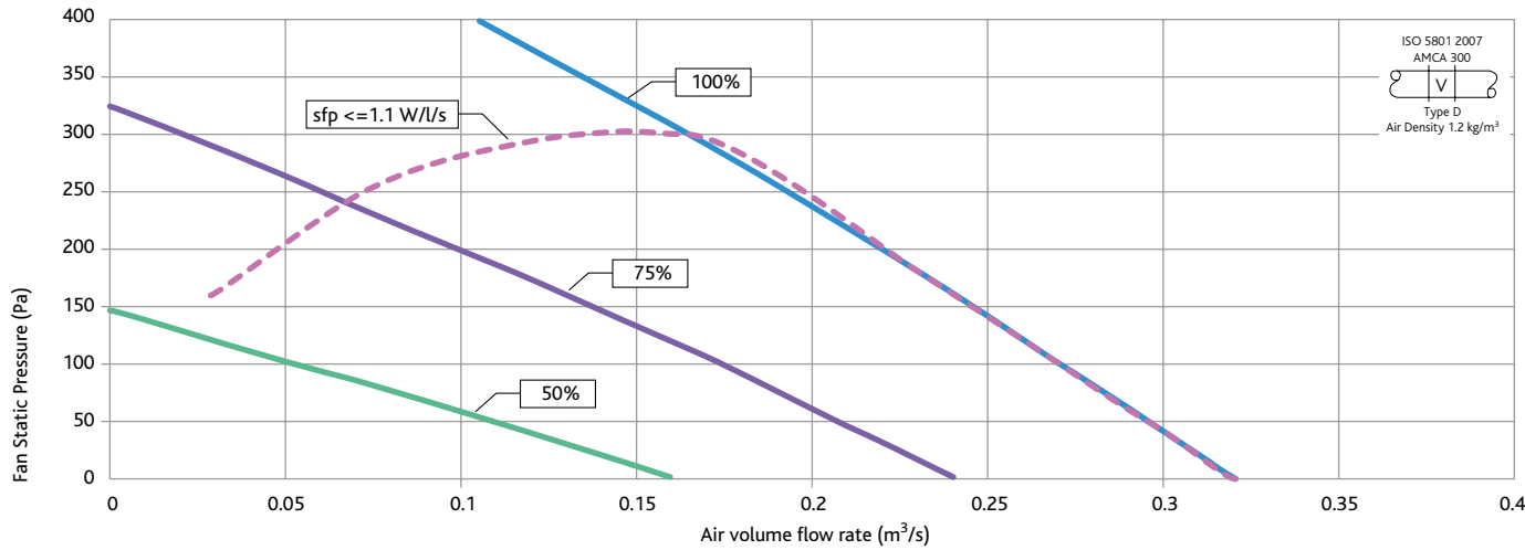
SUPPLY FAN SIZE DS4 - PERFORMANCE
