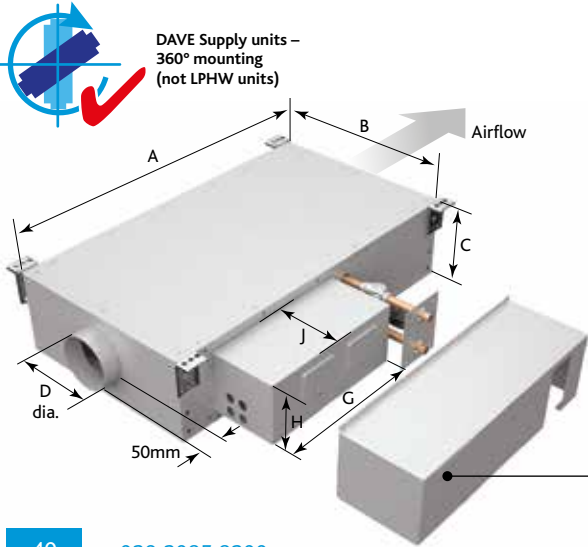
SUPPLY FAN SIZE DS7 - DATA LPHW 82/71 (Deg C)
