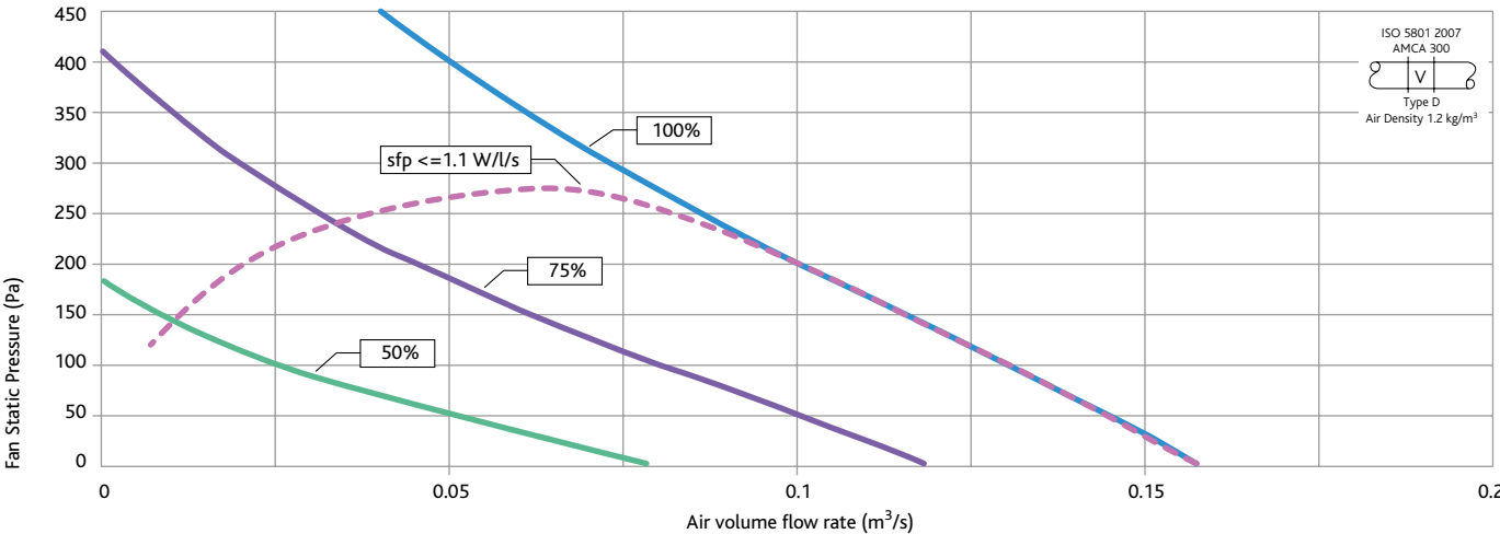
SUPPLY FAN SIZE DS2 - PERFORMANCE
