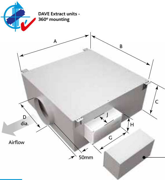
EXTRACT FAN SIZE DE6 - DIMENSIONS (mm)
