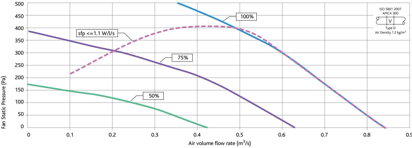
SUPPLY FAN SIZE DS6 - PERFORMANCE
