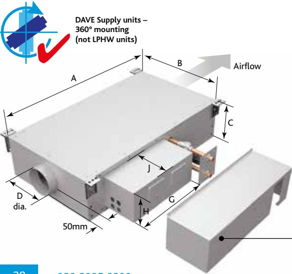
SUPPLY FAN SIZE DS5 - DATA LPHW 82/71 (Deg C)
