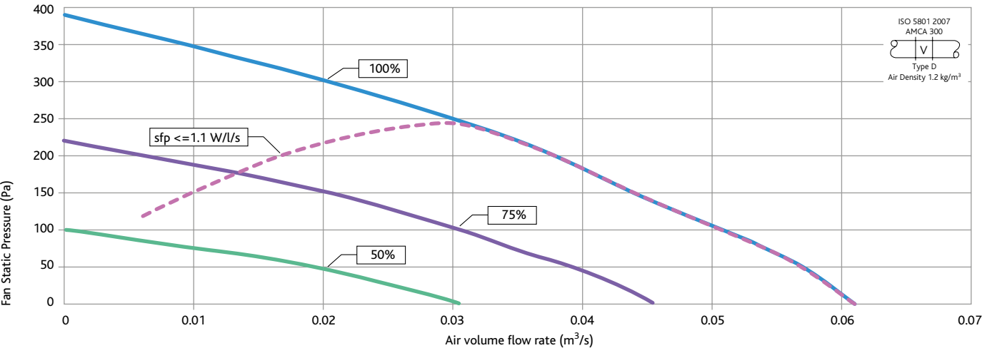
SUPPLY FAN SIZE DS1 - PERFORMANCE
