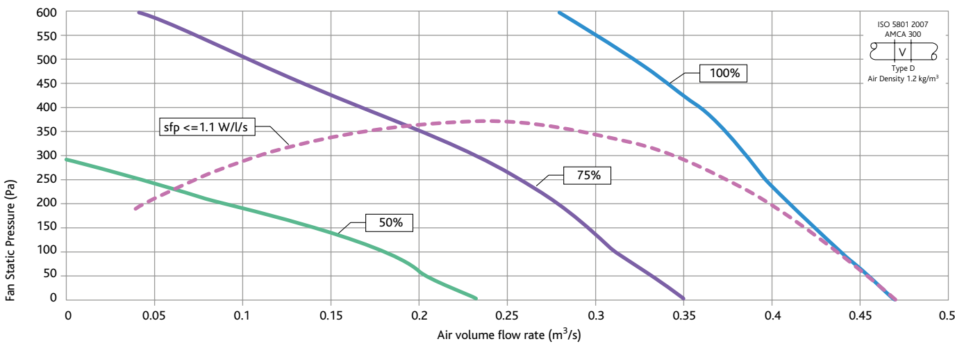
SUPPLY FAN SIZE DS4H - PERFORMANCE
