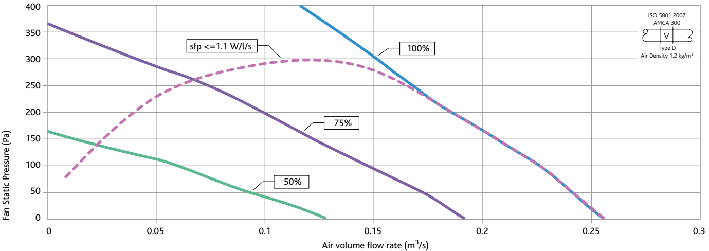
SUPPLY FAN SIZE DS3 - PERFORMANCE
