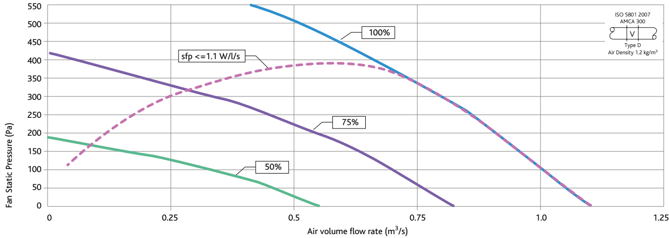
SUPPLY FAN SIZE DS7 - PERFORMANCE
