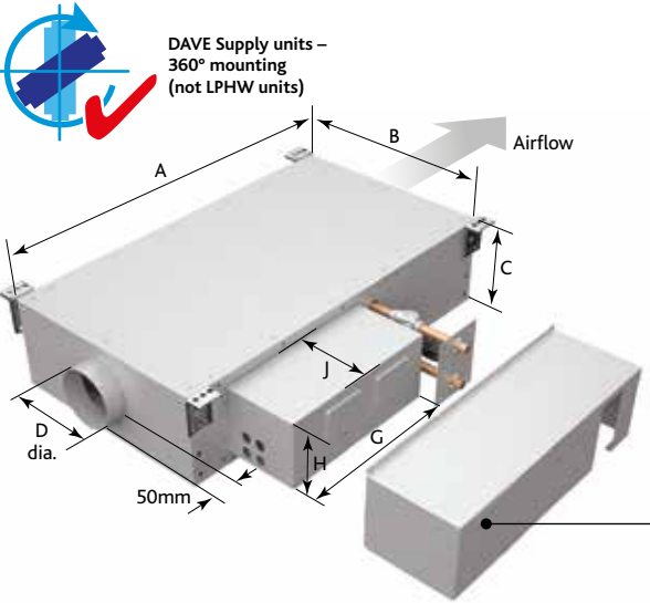
SUPPLY FAN SIZE DS4H - DATA LPHW 82/71 (Deg C)
