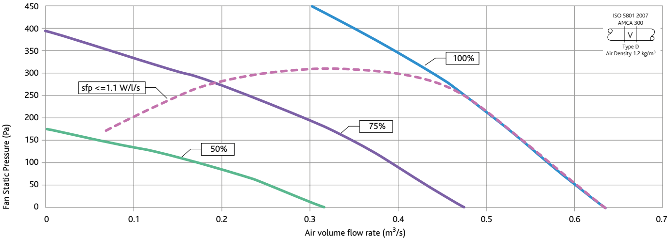
SUPPLY FAN SIZE DS5 - PERFORMANCE
