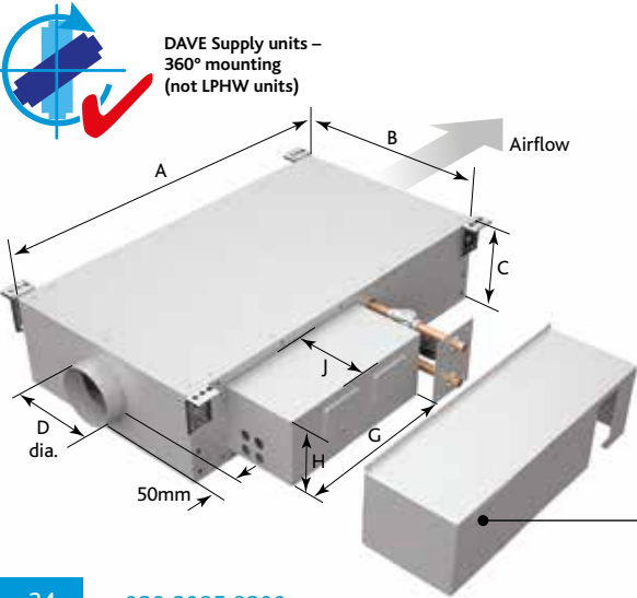
SUPPLY FAN SIZE DS2H - DATA LPHW 82/71 (Deg C)
