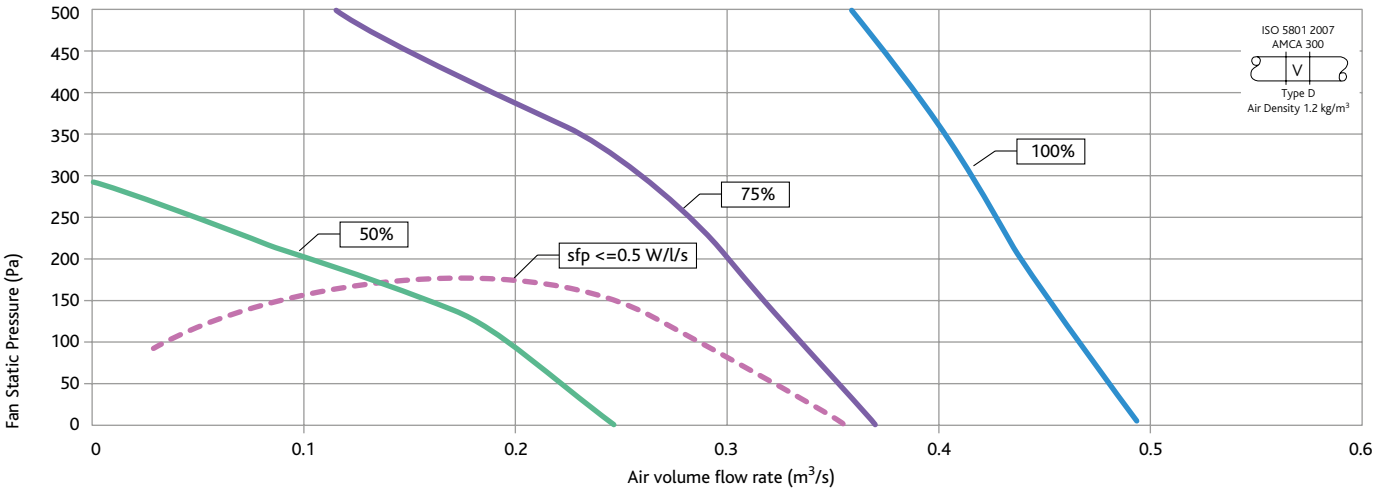
EXTRACT FAN SIZE DE4H - PERFORMANCE
