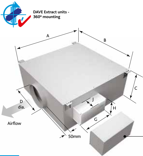
EXTRACT FAN SIZE DE4H - DIMENSIONS (mm)
