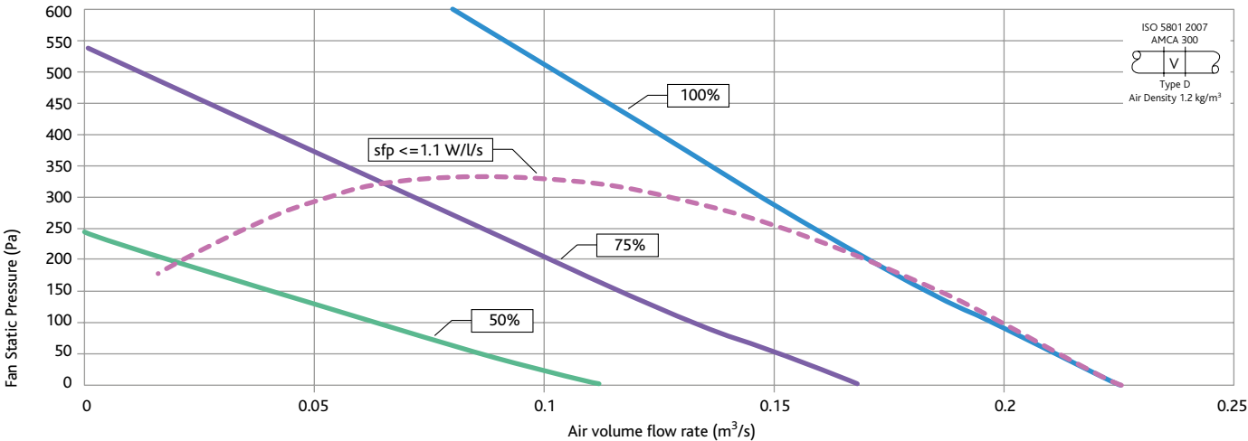
SUPPLY FAN SIZE DS2H - PERFORMANCE
