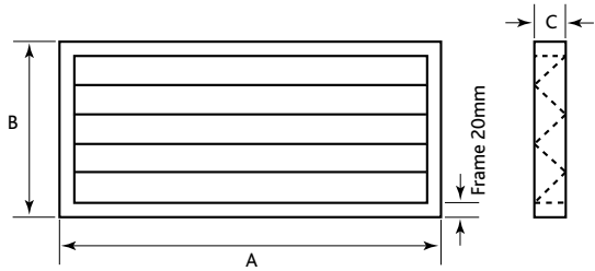
FILTERS - G3/G4/F7 (SITE REPLACEMENT)
