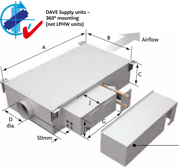
SUPPLY FAN SIZE DS3 - DATA LPHW 82/71 (Deg C)
