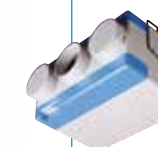
ES OPUS DC (up to 110l/s) High performance, low noise ceiling void extract range with very low profile complete with Ecosmart control.
