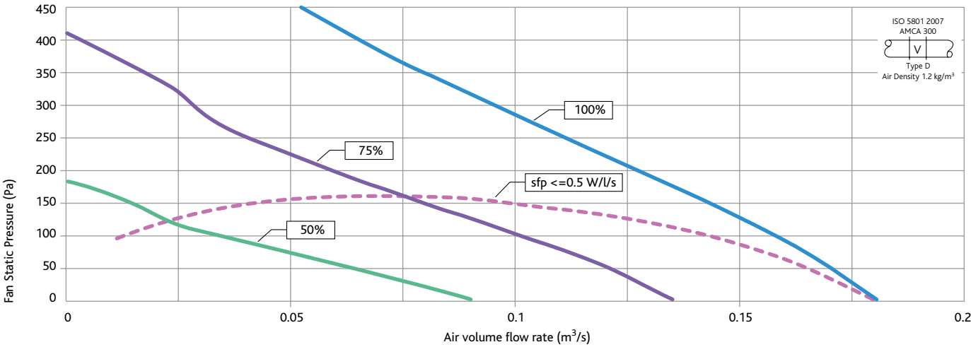
EXTRACT FAN SIZE DE2 - PERFORMANCE
