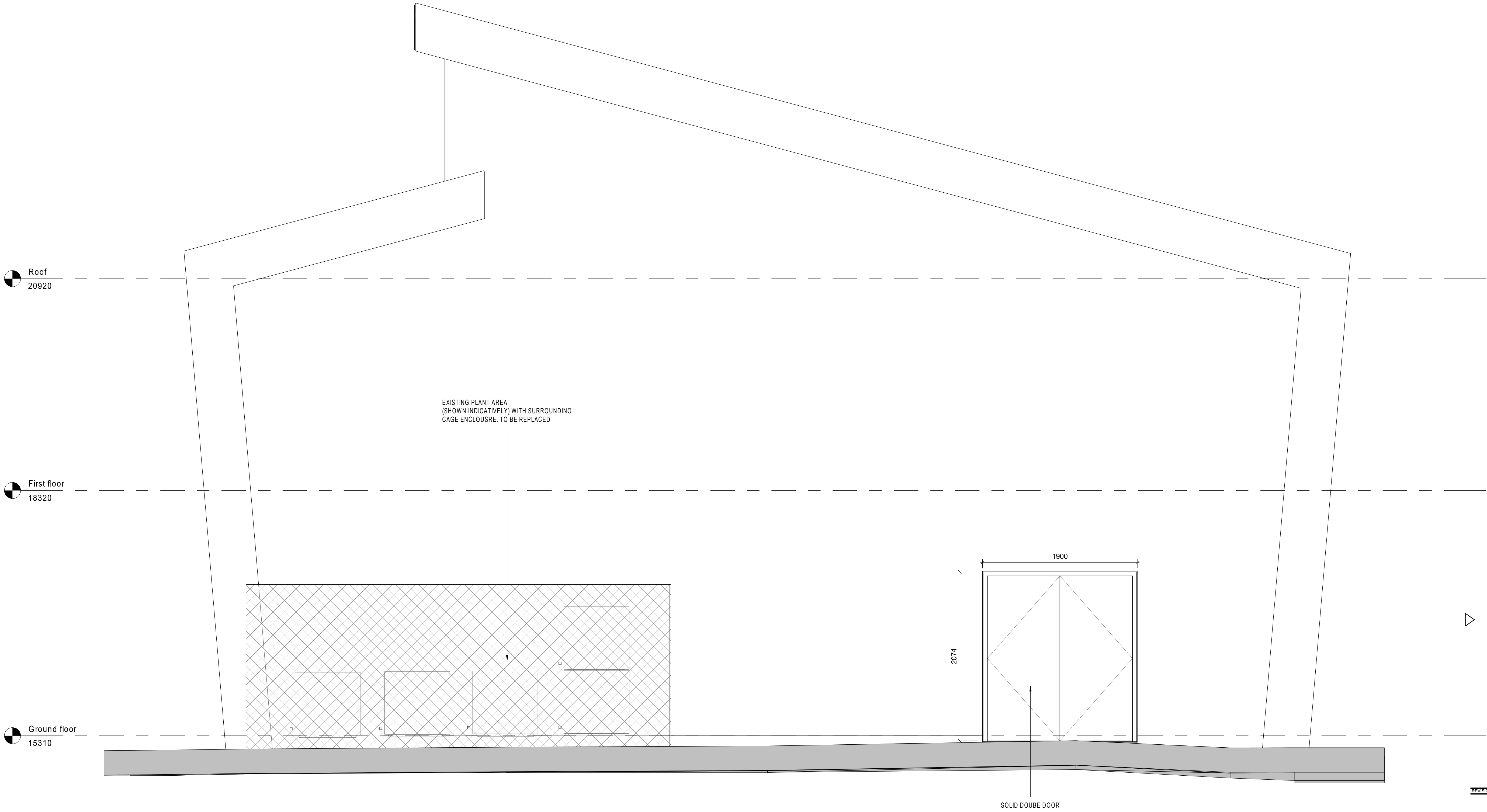
1 EXISITNG ELEVATION - BACK 1 : 25
