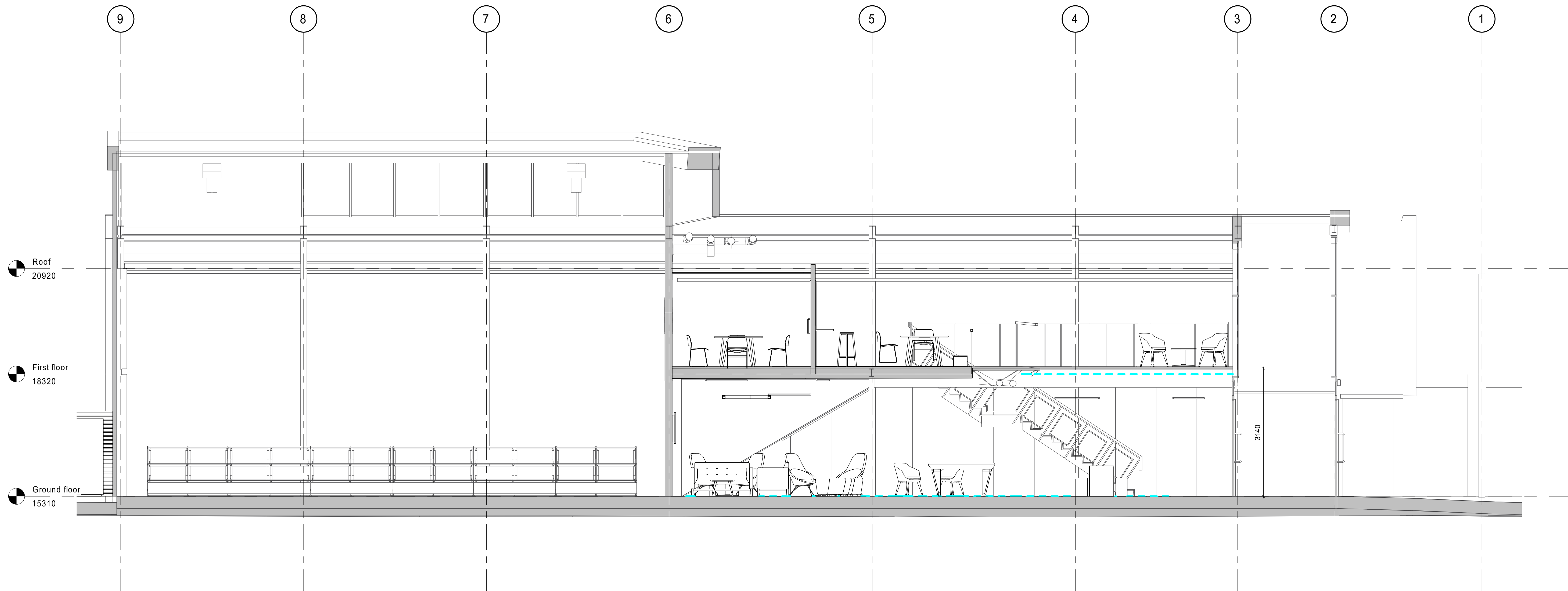
1 PROPOSED LONG SECTION CC 1 : 50
