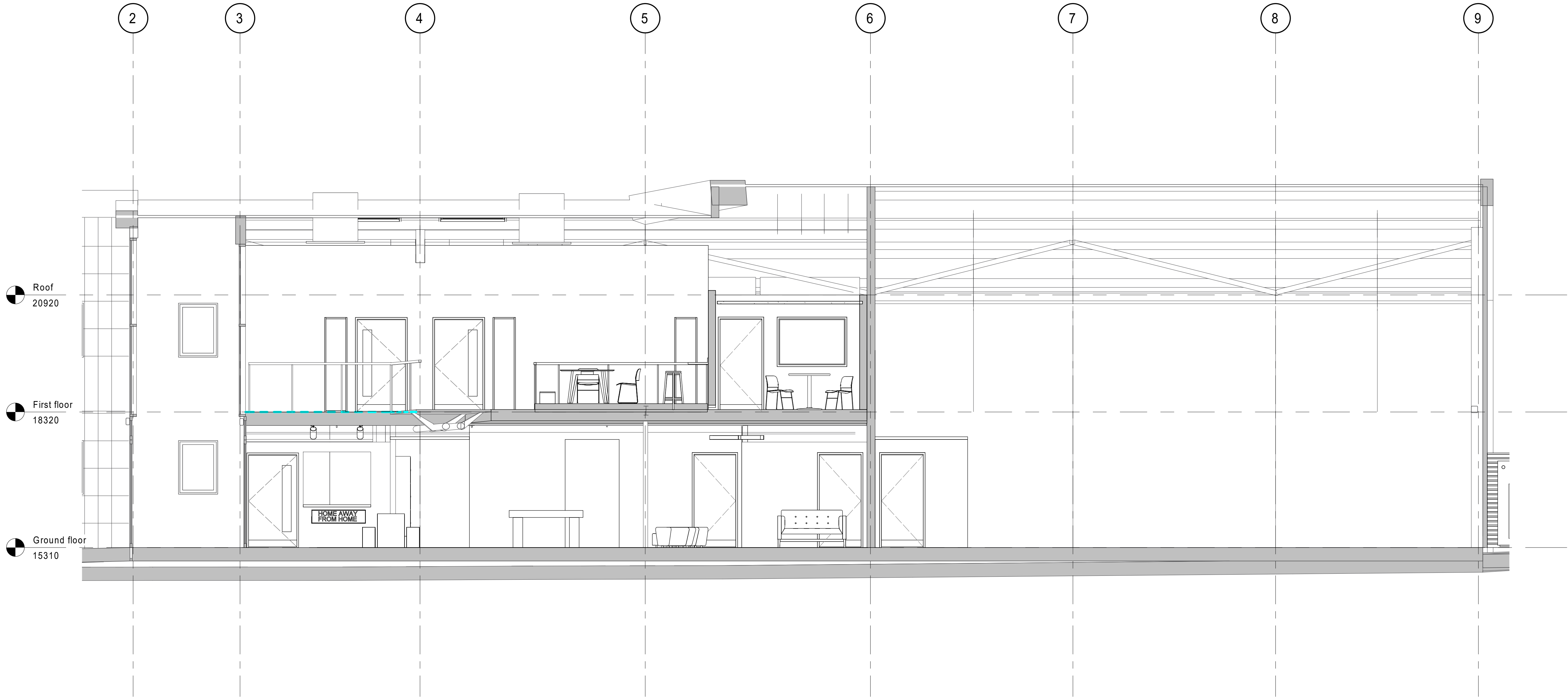
1 PROPOSED LONG SECTION DD 1 : 50
