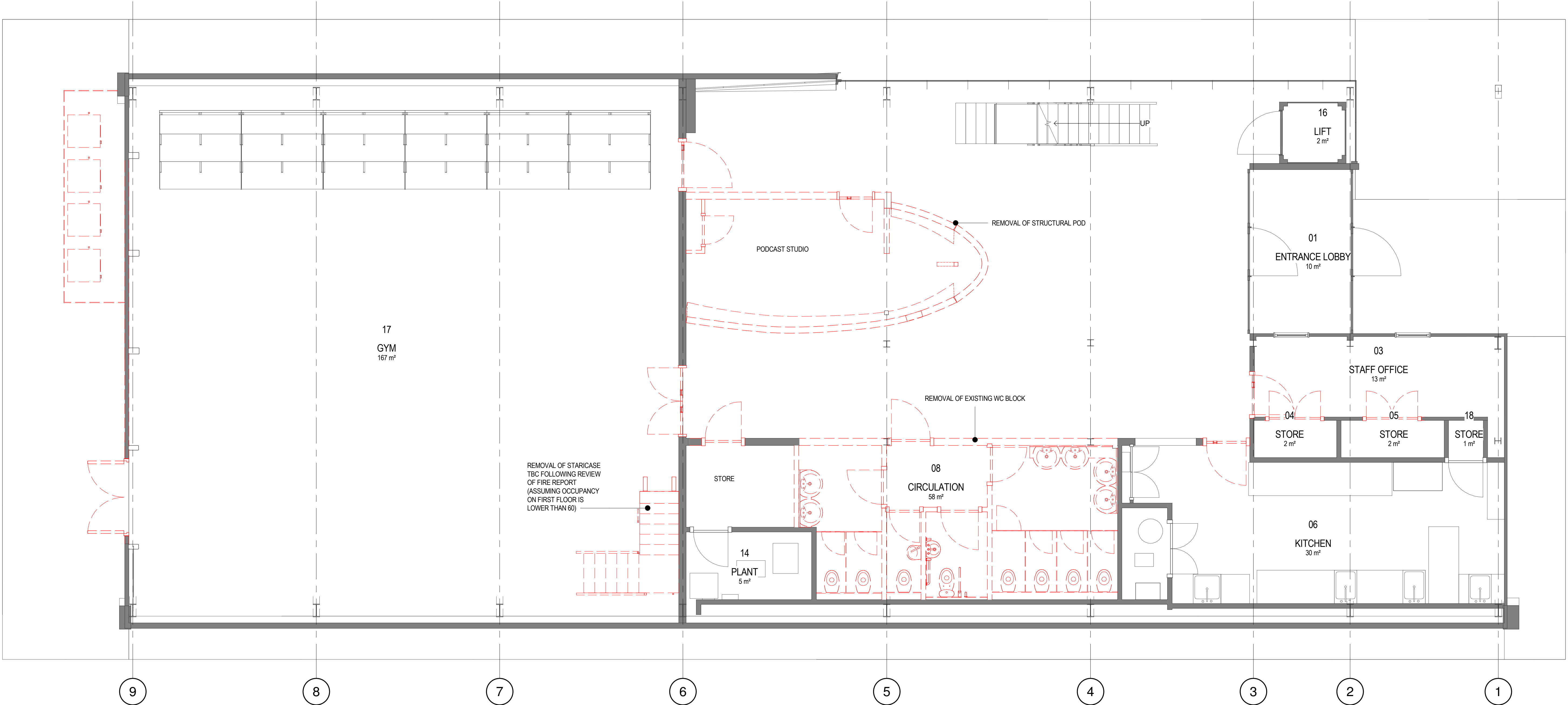
1 DEMOLITION PLAN - GROUND FLOOR 1 : 50
