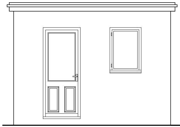
1:50 SOUTH ELEVATION
