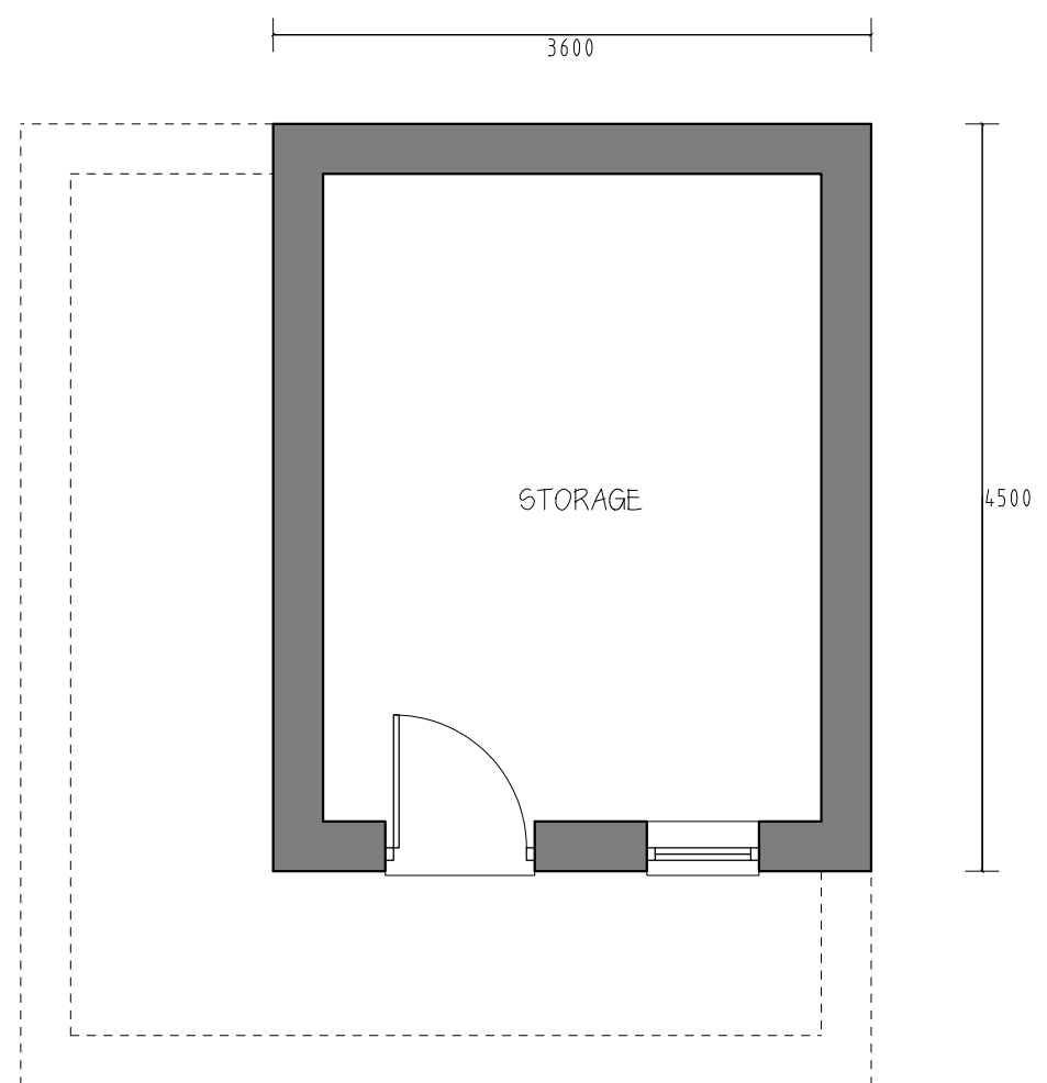
1:50 FLOOR PLAN
