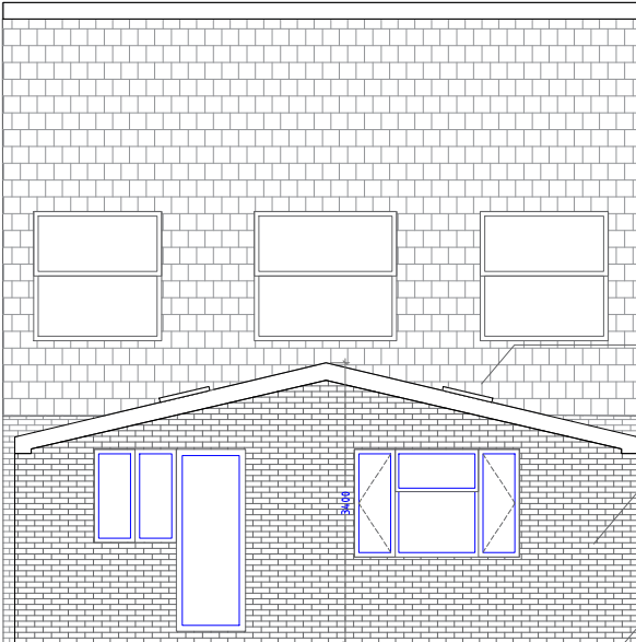
PROPOSED BACK ELEVATION PLAN
