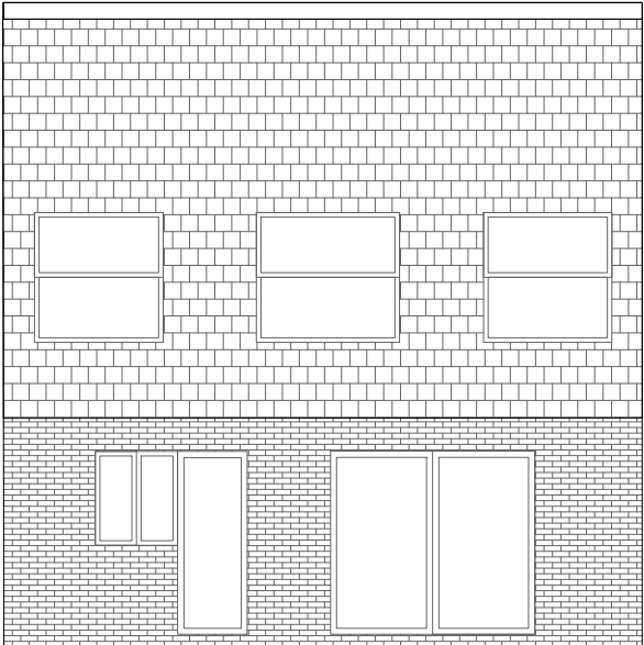
EXISTING BACK ELEVATION PLAN
