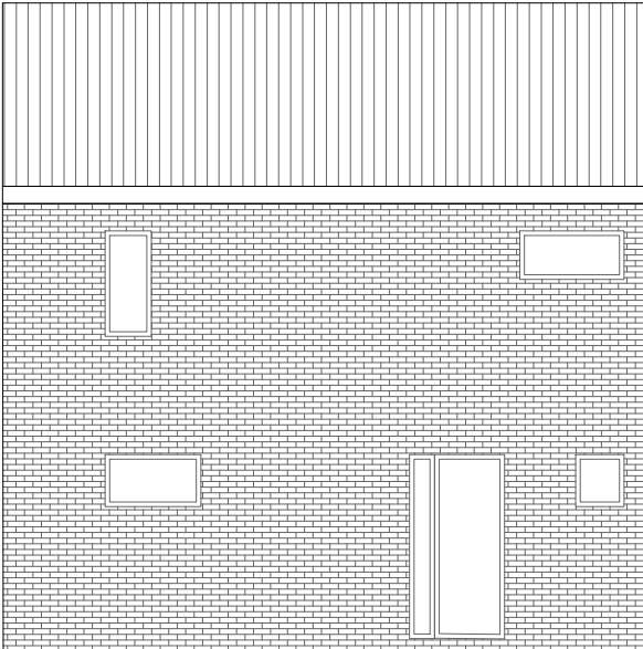
PROPOSED FRONT ELEVATION PLAN
