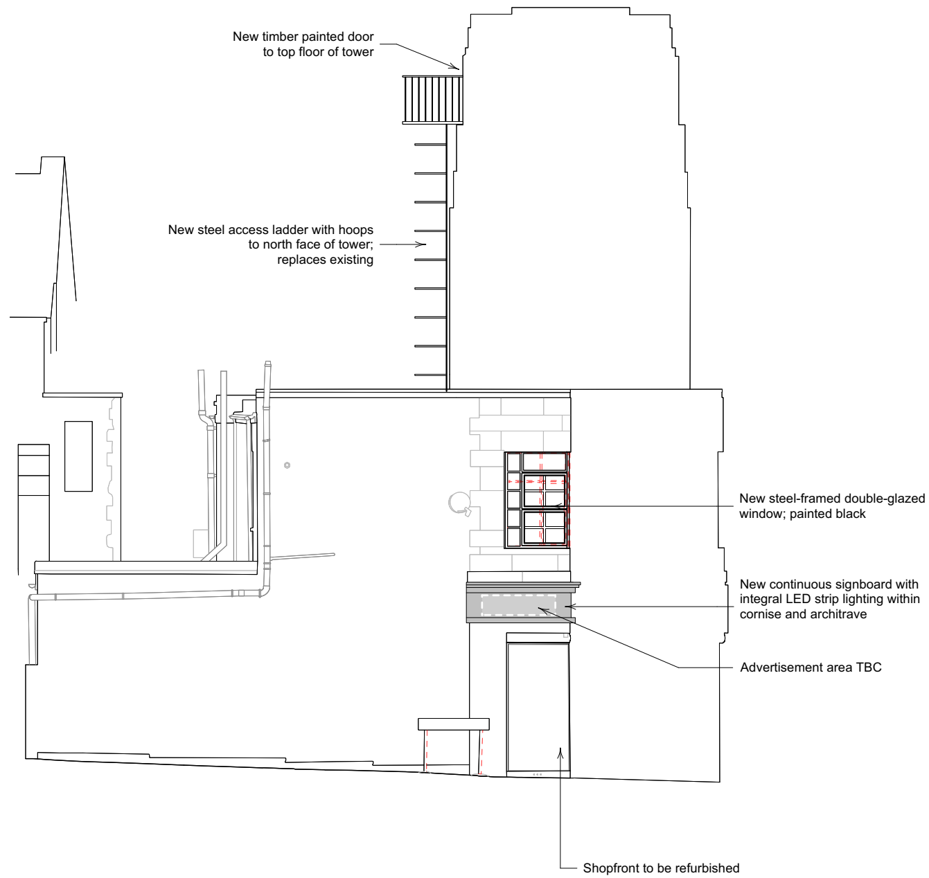
01 South Elevation B3 1:100@A3; 1:50@A1
