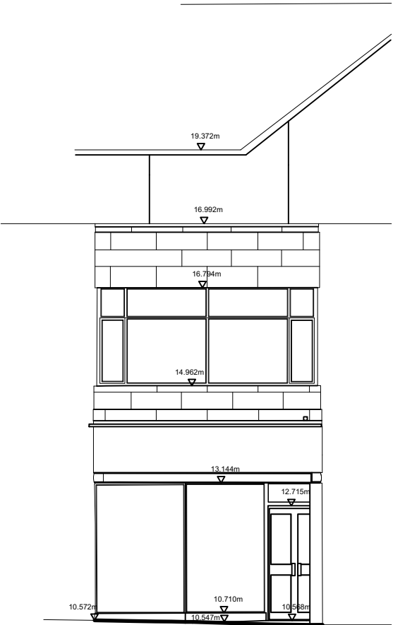
02 South Elevation B4 1:100@A3; 1:50@A1
