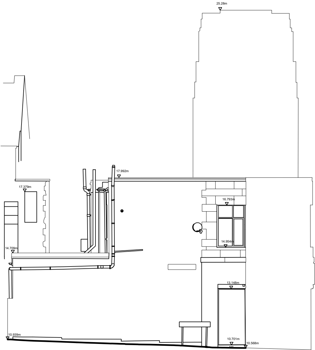
01 South Elevation B3 1:100@A3; 1:50@A1
