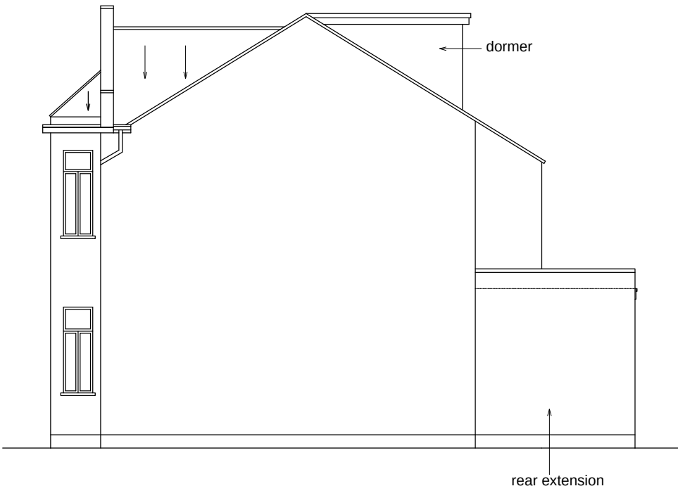
Side elevation (from South) Scale: 1/100
