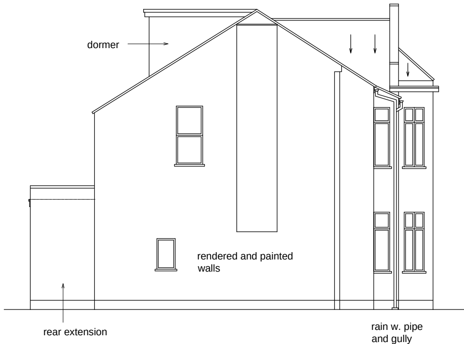
Side elevation (from North) Scale: 1/100
