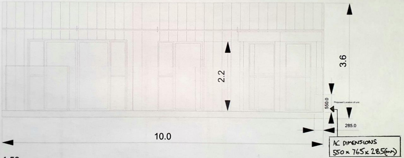
East Elevation
