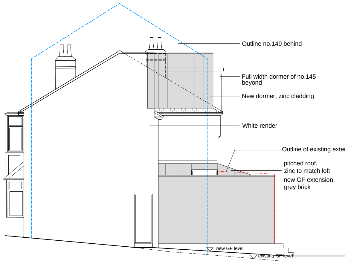
SIDE ELEVATION
