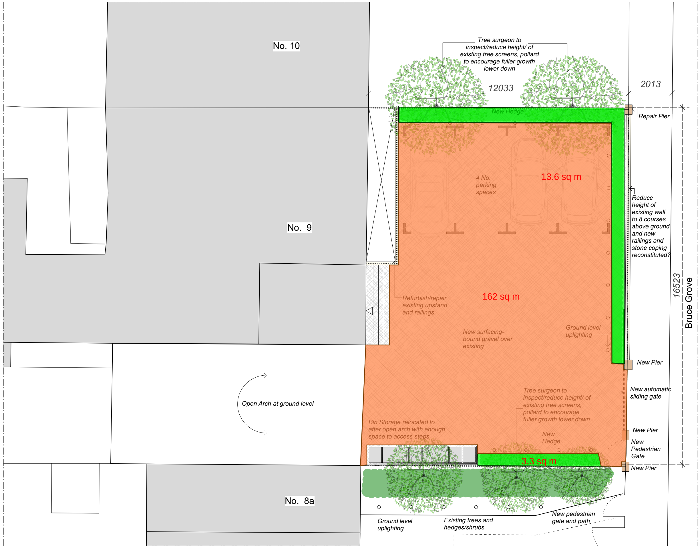
01 9 Bruce Grove Plan BG09-02 1:100@A3; 1:50@A1
