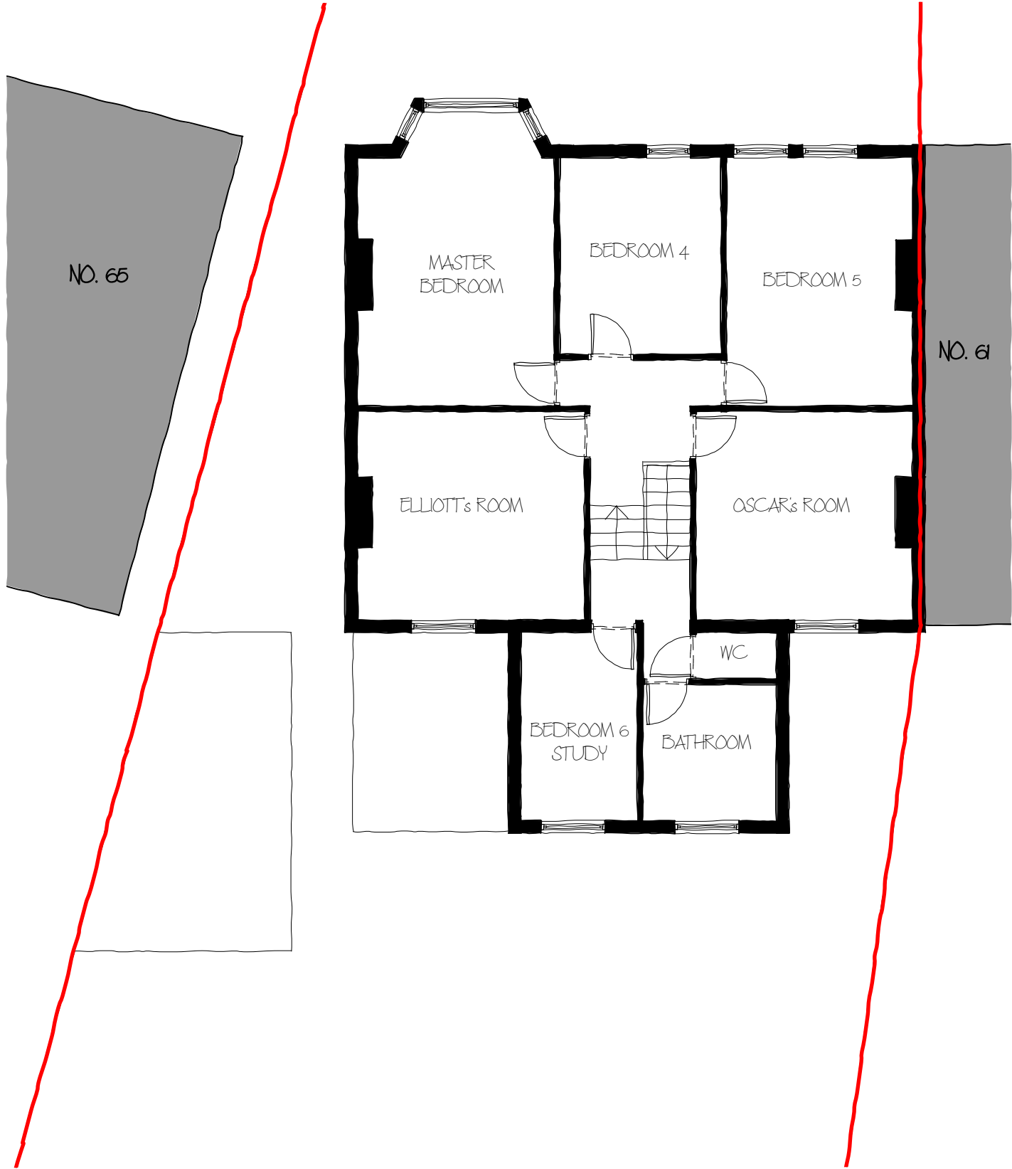
01 - Existing First Floor Plan 1:100@A3
