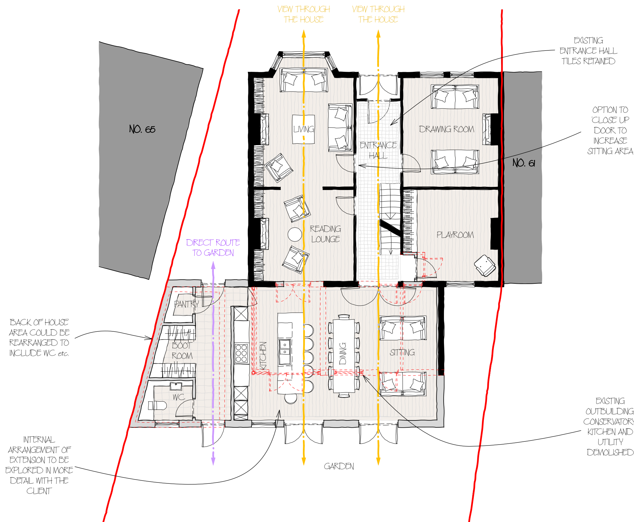
00 - Proposed Ground Floor Plan 1:100@A3
