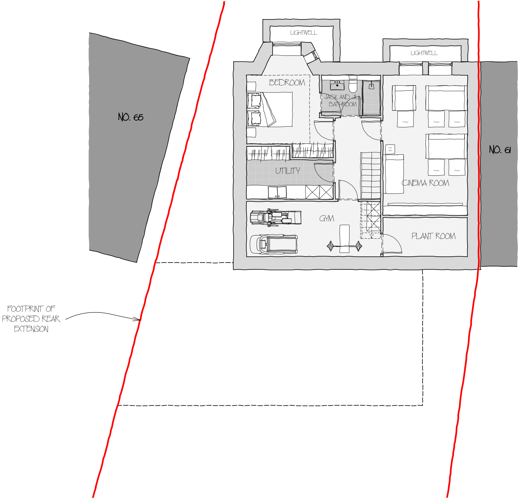
00 - Proposed Basement Floor Plan 1:100@A3
