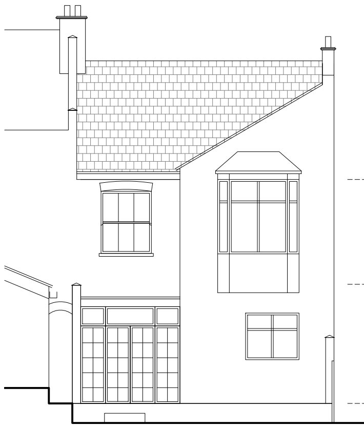
REAR ELEVATION
