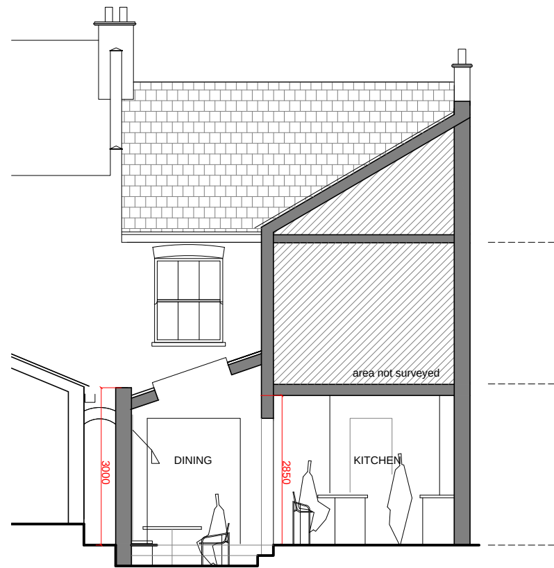
SECTION AA
