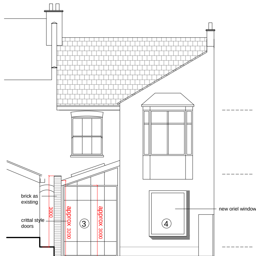
REAR ELEVATION
