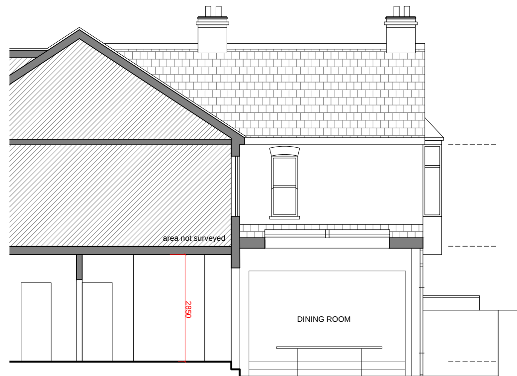
SECTION BB
