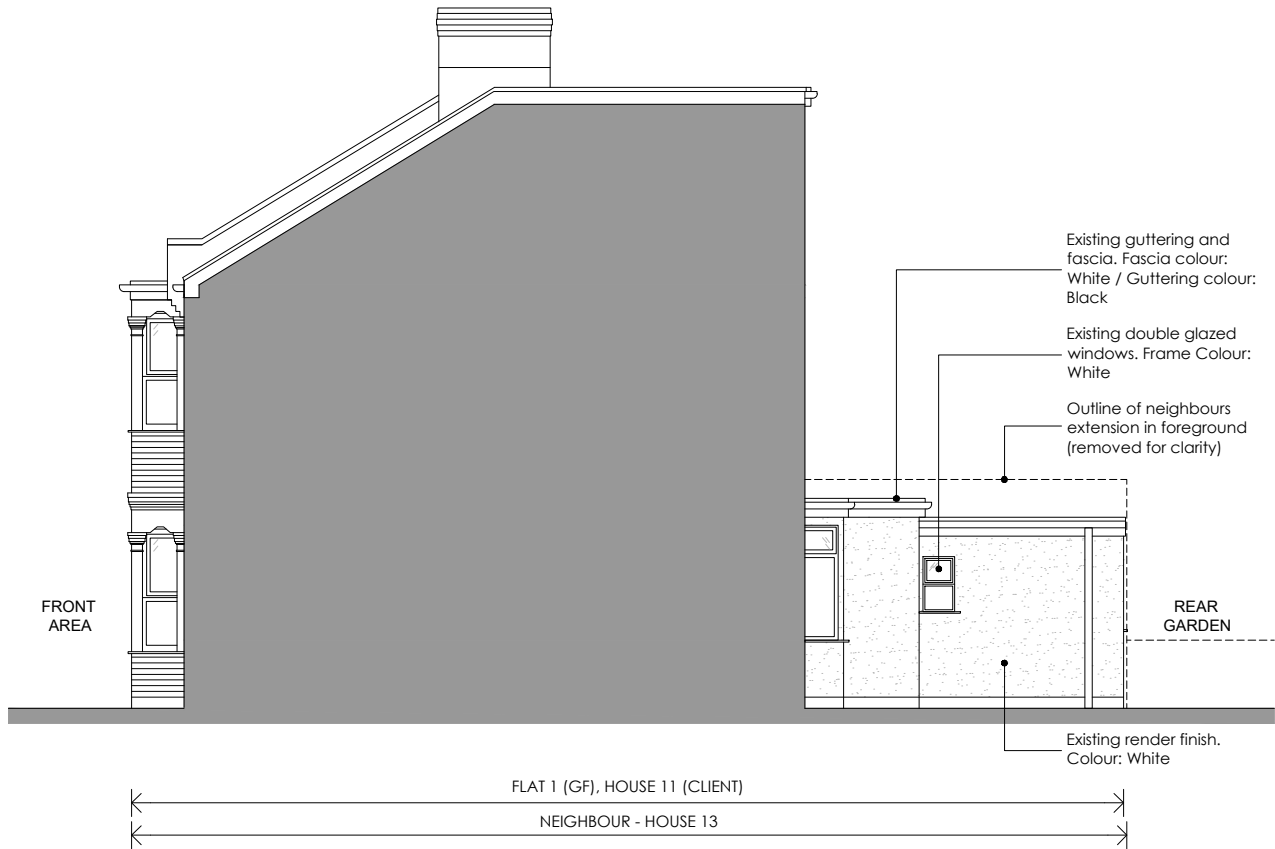
EXISTING LHS ELEVATION
