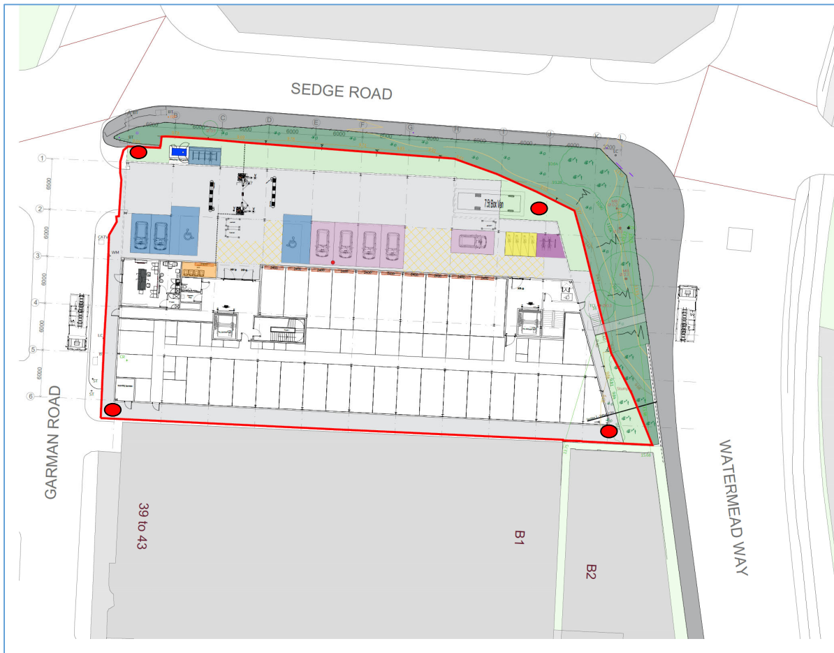
Figure 4 – Vibration monitoring equipment locations
