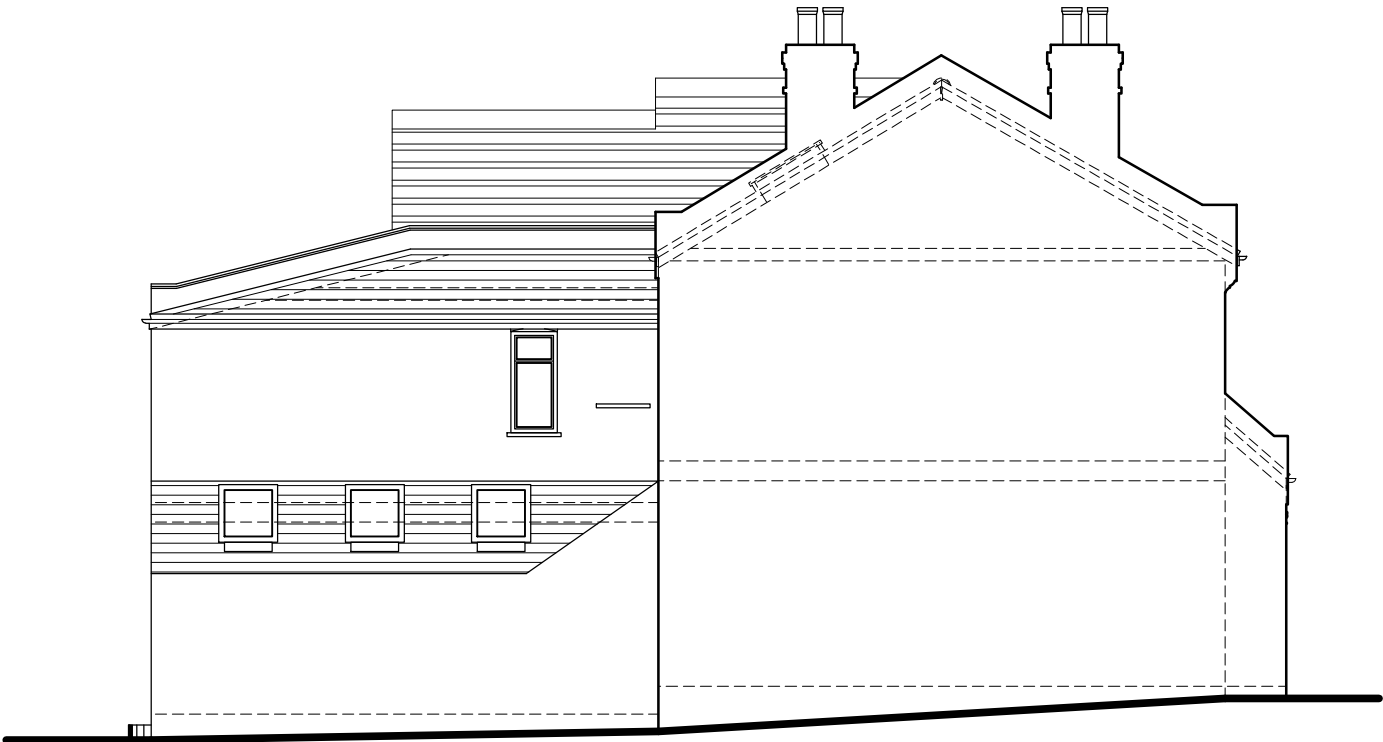
Proposed Side Elevation 01
