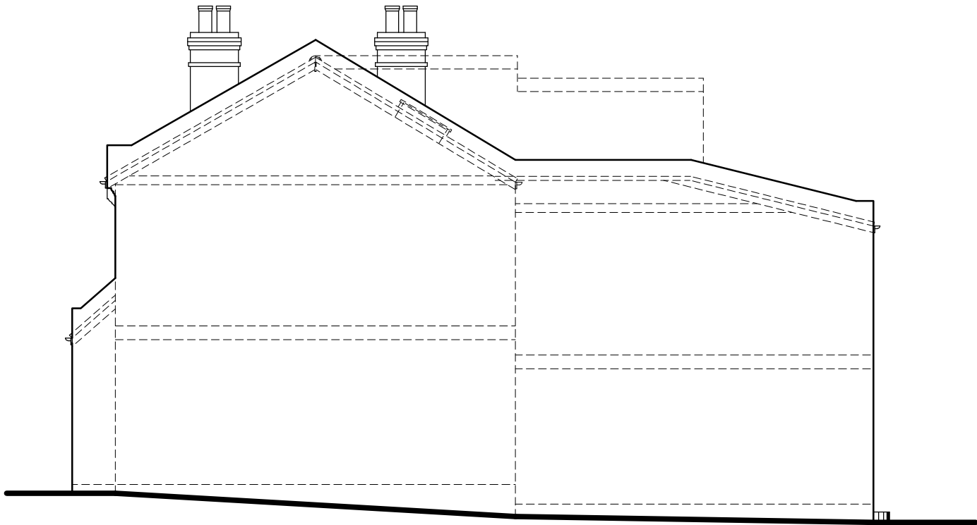
Side Elevation 02
