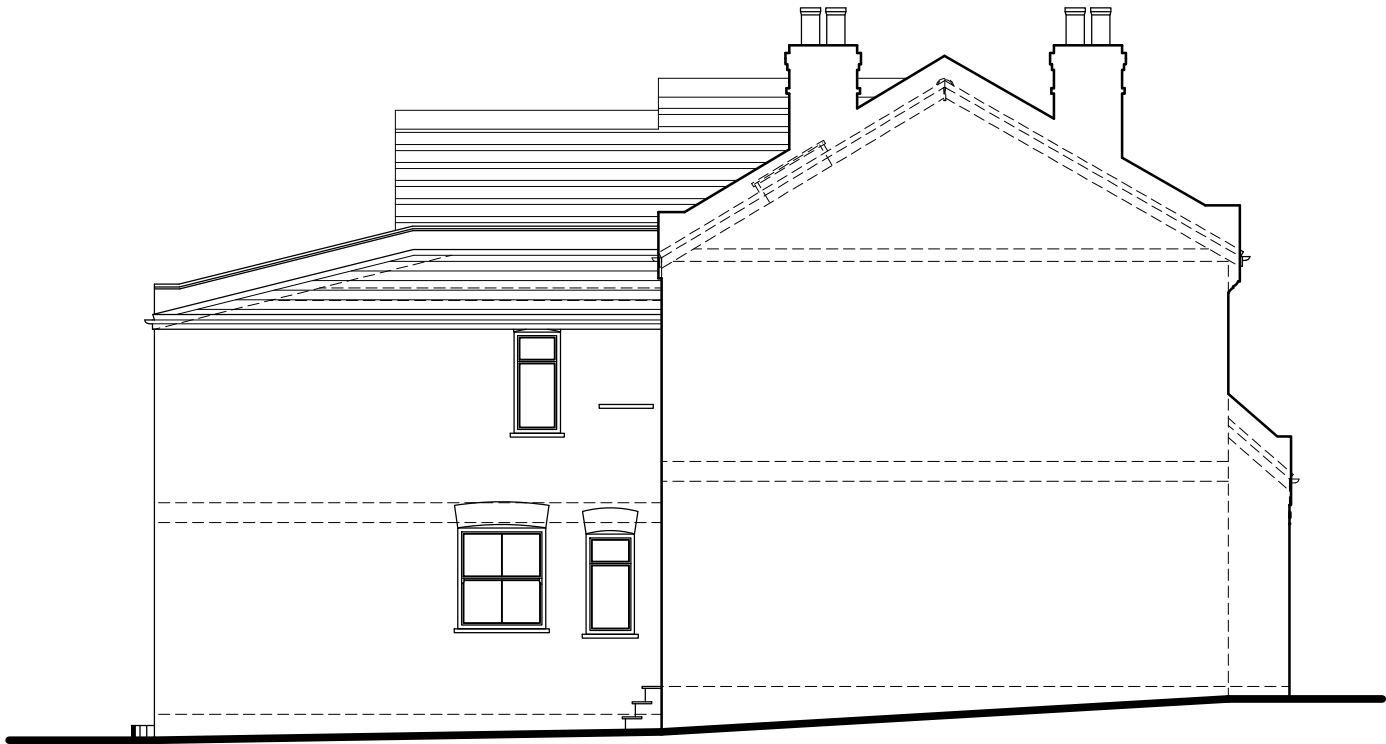
Side Elevation 01
