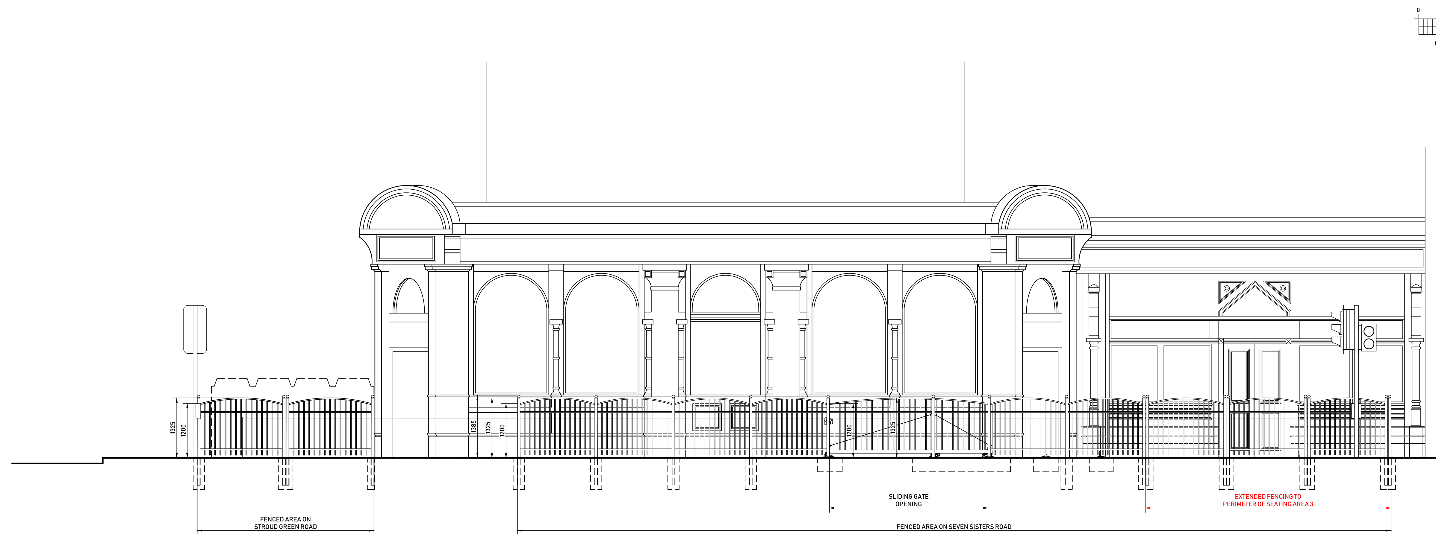
ELEVATION 1-1. SEVEN SISTERS ROAD ELEVATION.
