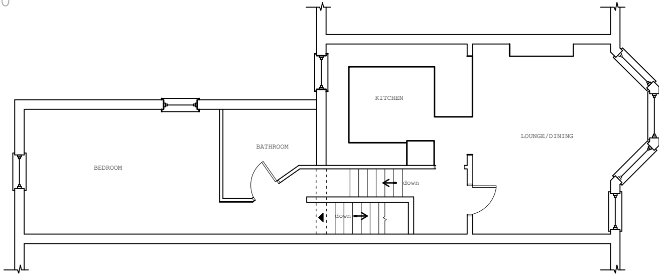
2 FIRST FLOOR 1:100
