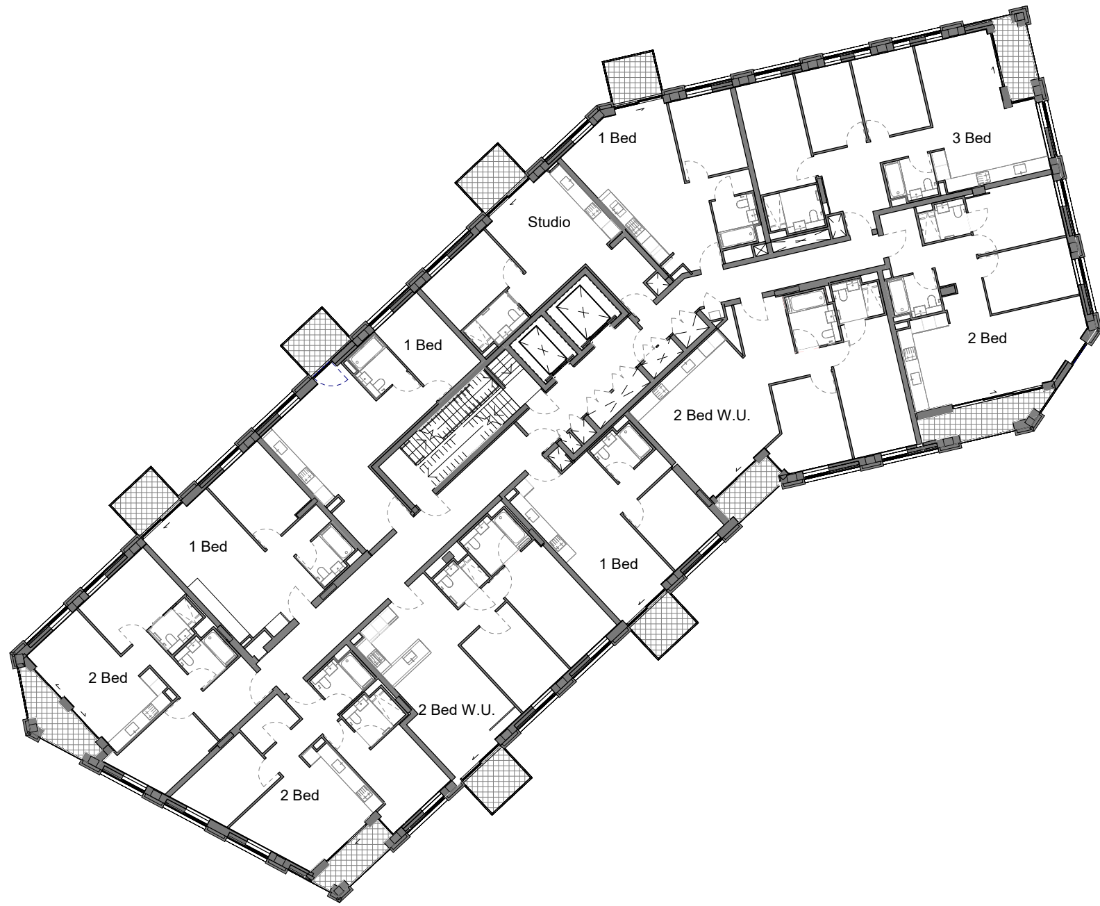
BUILDING 2
