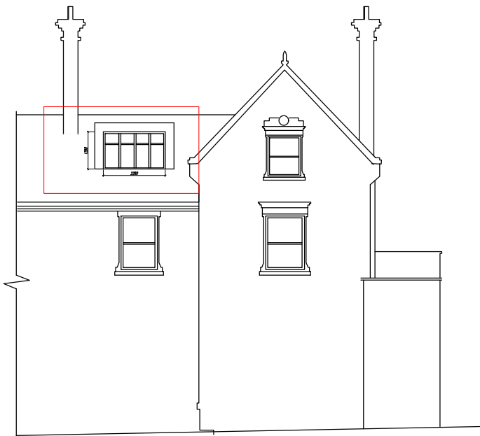
01 Existing Front Elevation
