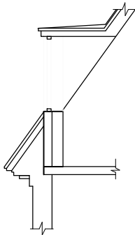
Section A-A Existing
