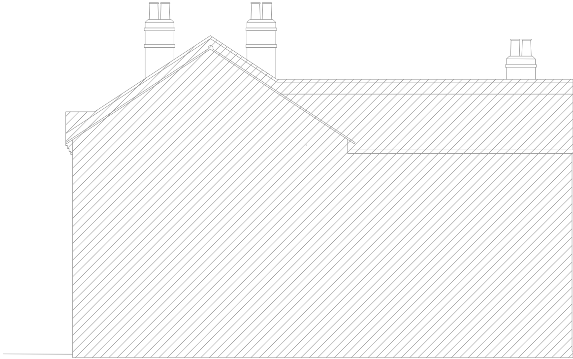
050.3 SIDE ELEVATION AS EXISTING
