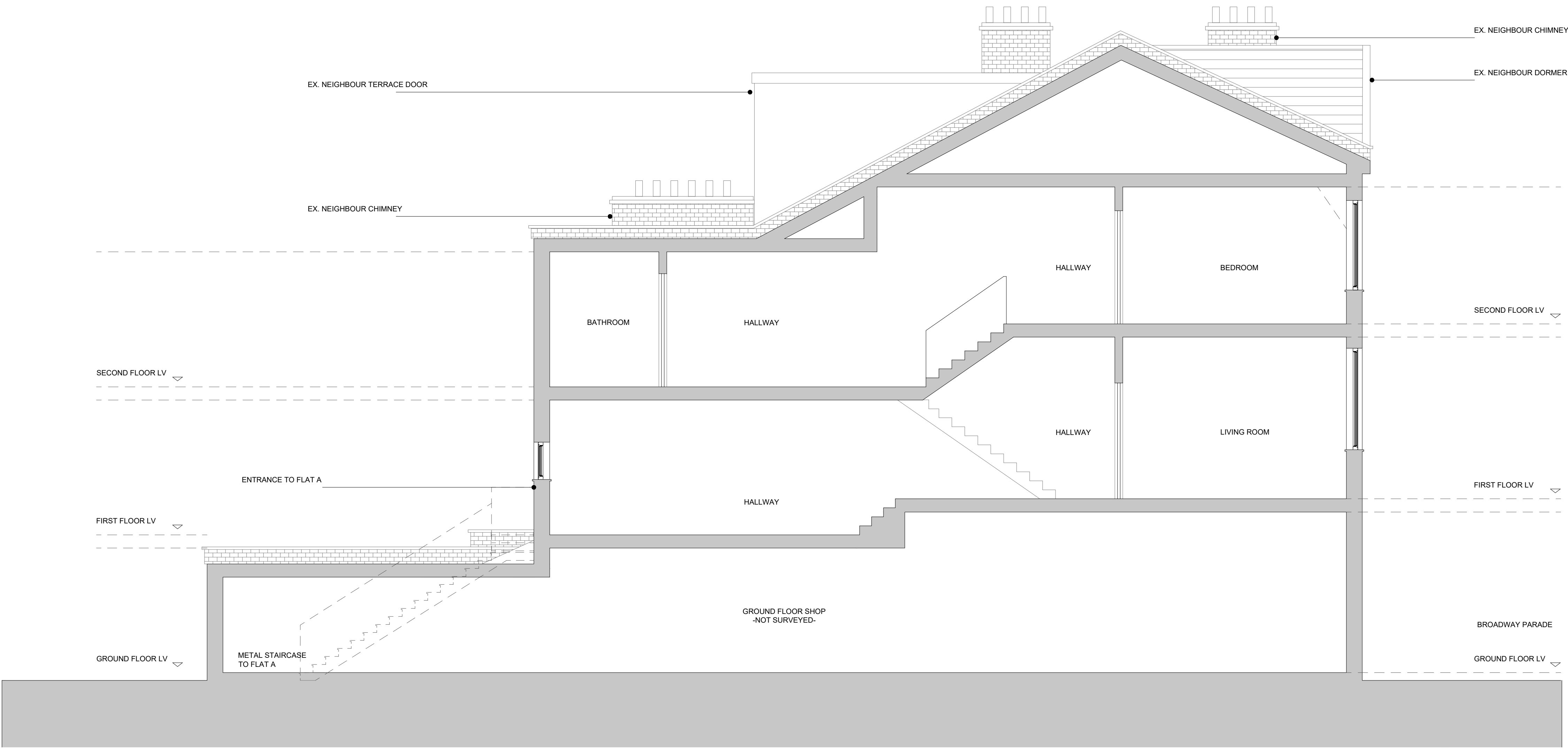
1 Existing Section AA Scale 1:50
