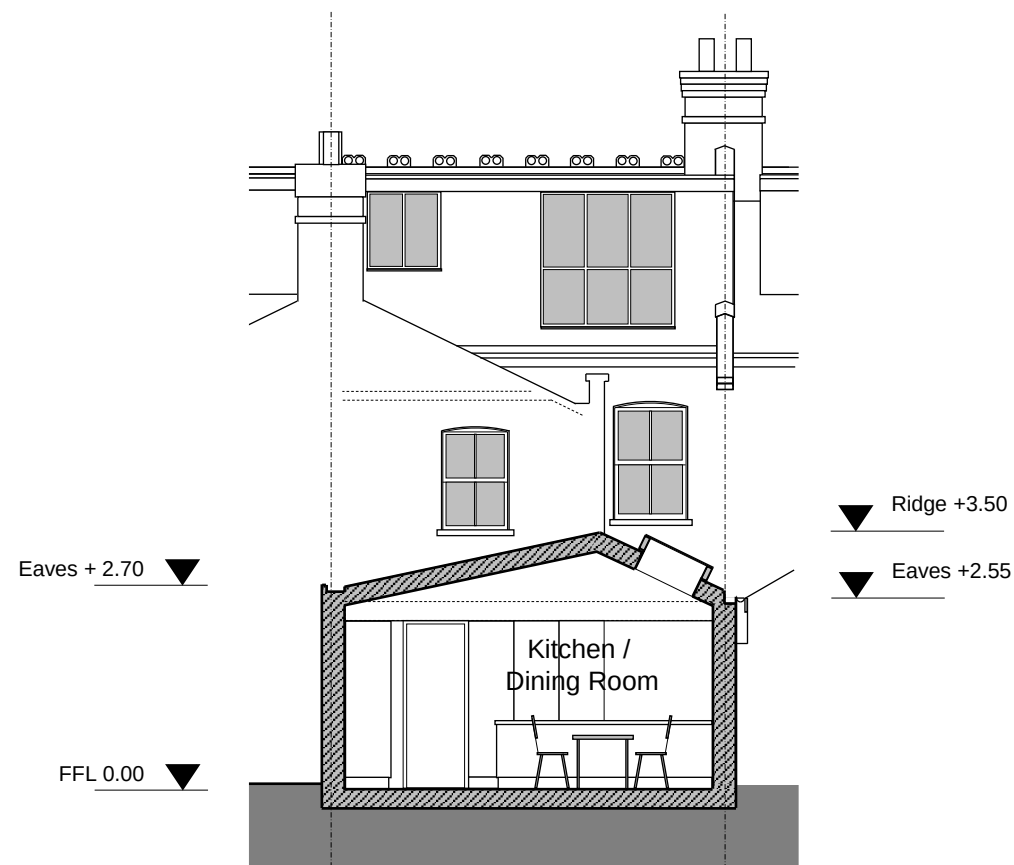
Section E-E
