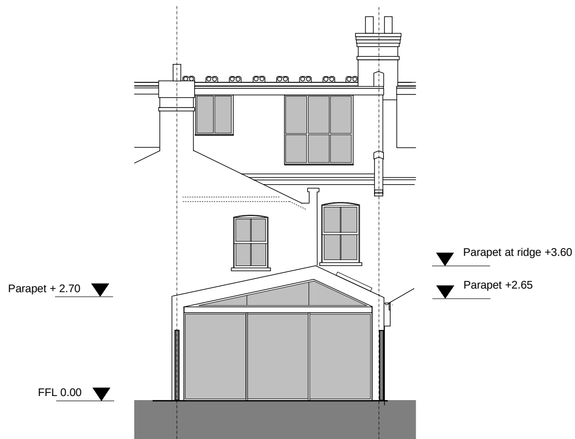
Rear Elevation – Section D-D
