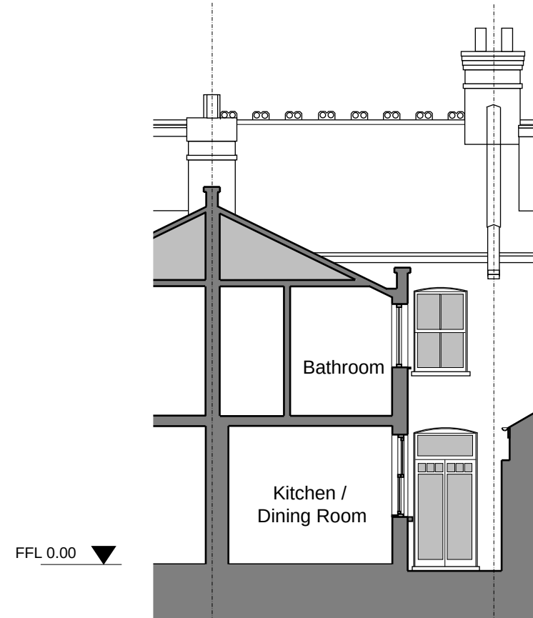
Section C-C
