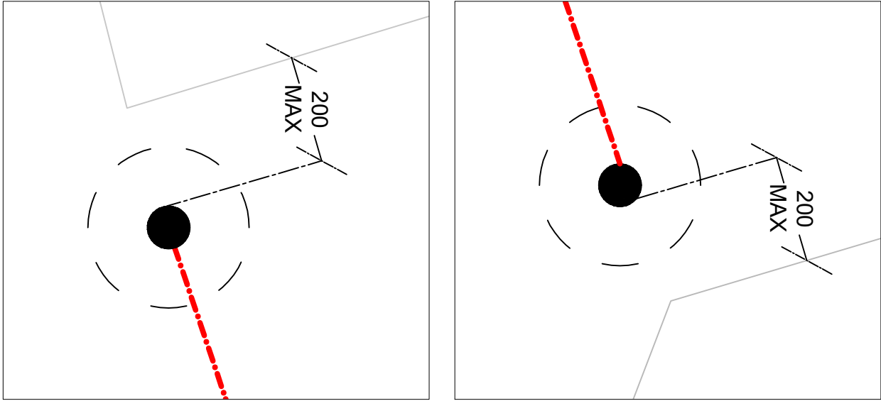
SP 7A Detail Scale 1:10 SP 7B Detail Scale 1:10
