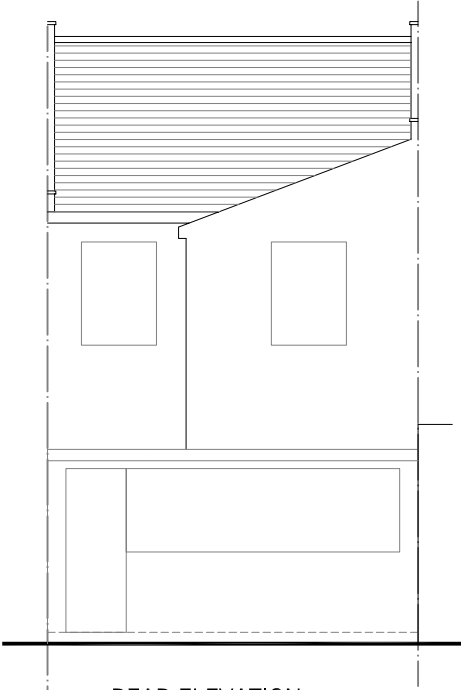
REAR ELEVATION
