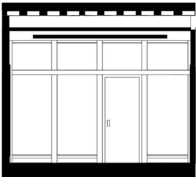
3 CC-00-033-Meeting Room-Elevation-N 1 : 50
