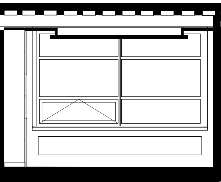
5 CC-00-033-Meeting Room-Elevation-S 1 : 50
