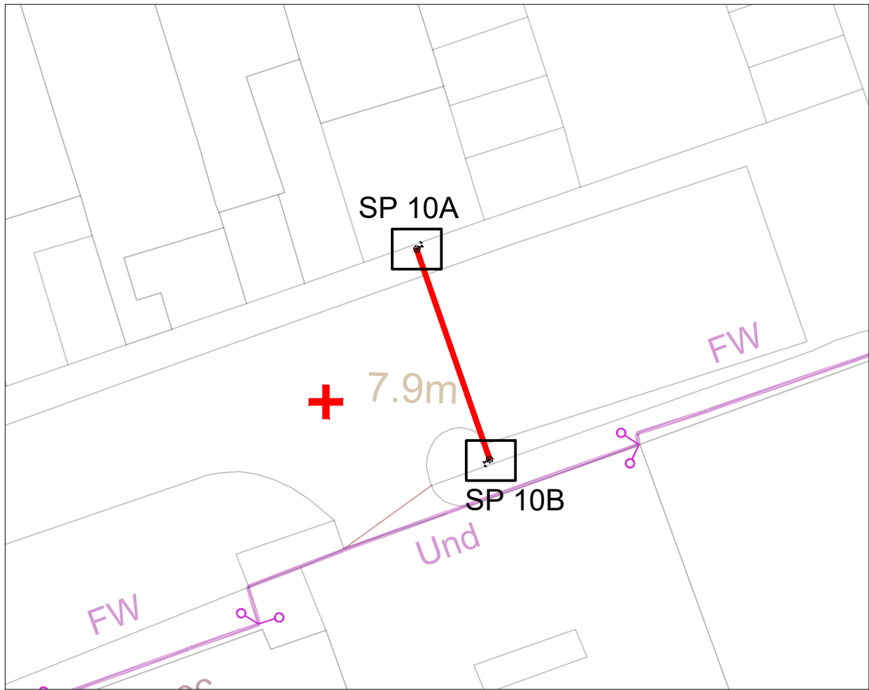
SP 10 LOCATION PLAN Scale 1:250
