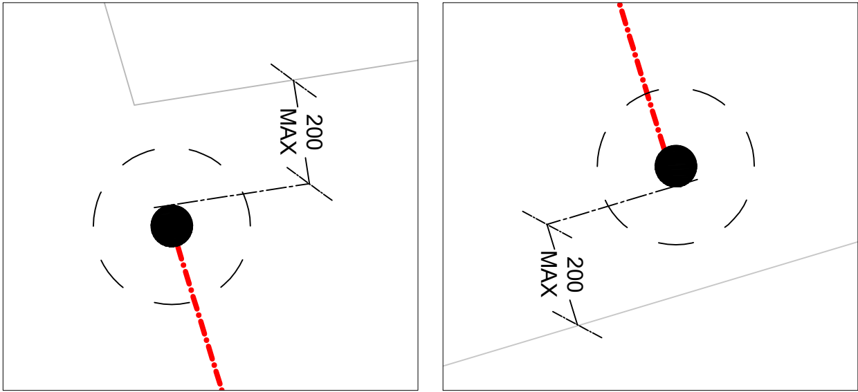
SP 9A Detail Scale 1:10 SP 9B Detail Scale 1:10
