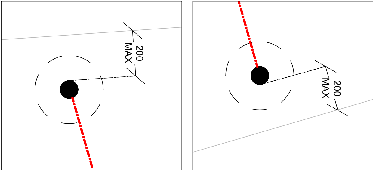
SP 3A Detail Scale 1:10
